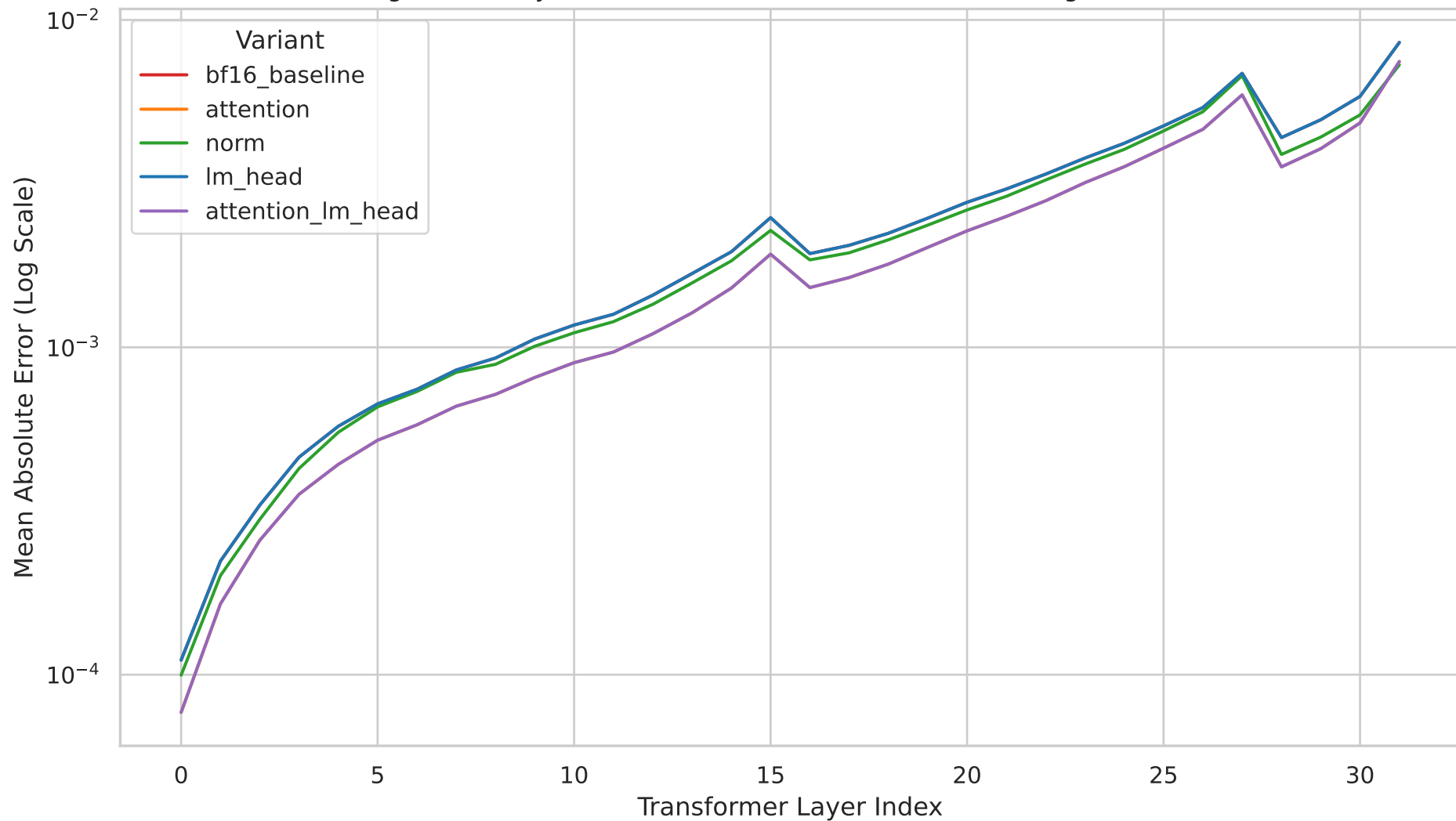
Figure M3. Layer-wise Hidden-State MAE vs FP32 (Divergent Cases)
