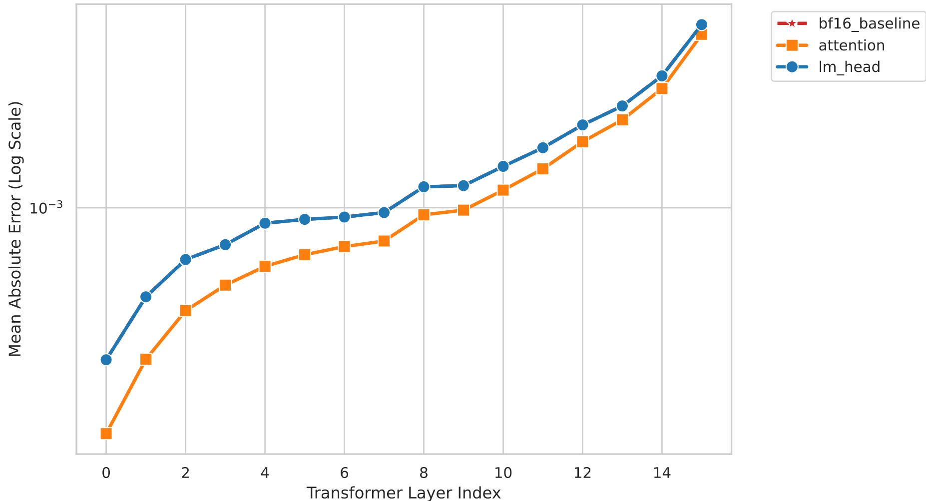
Figure M3. Layer-wise Hidden-State MAE vs FP32 Model: Llama-3.2-1B | Dataset: cmmlu | Base: bfloat16 (Divergent Cases)
