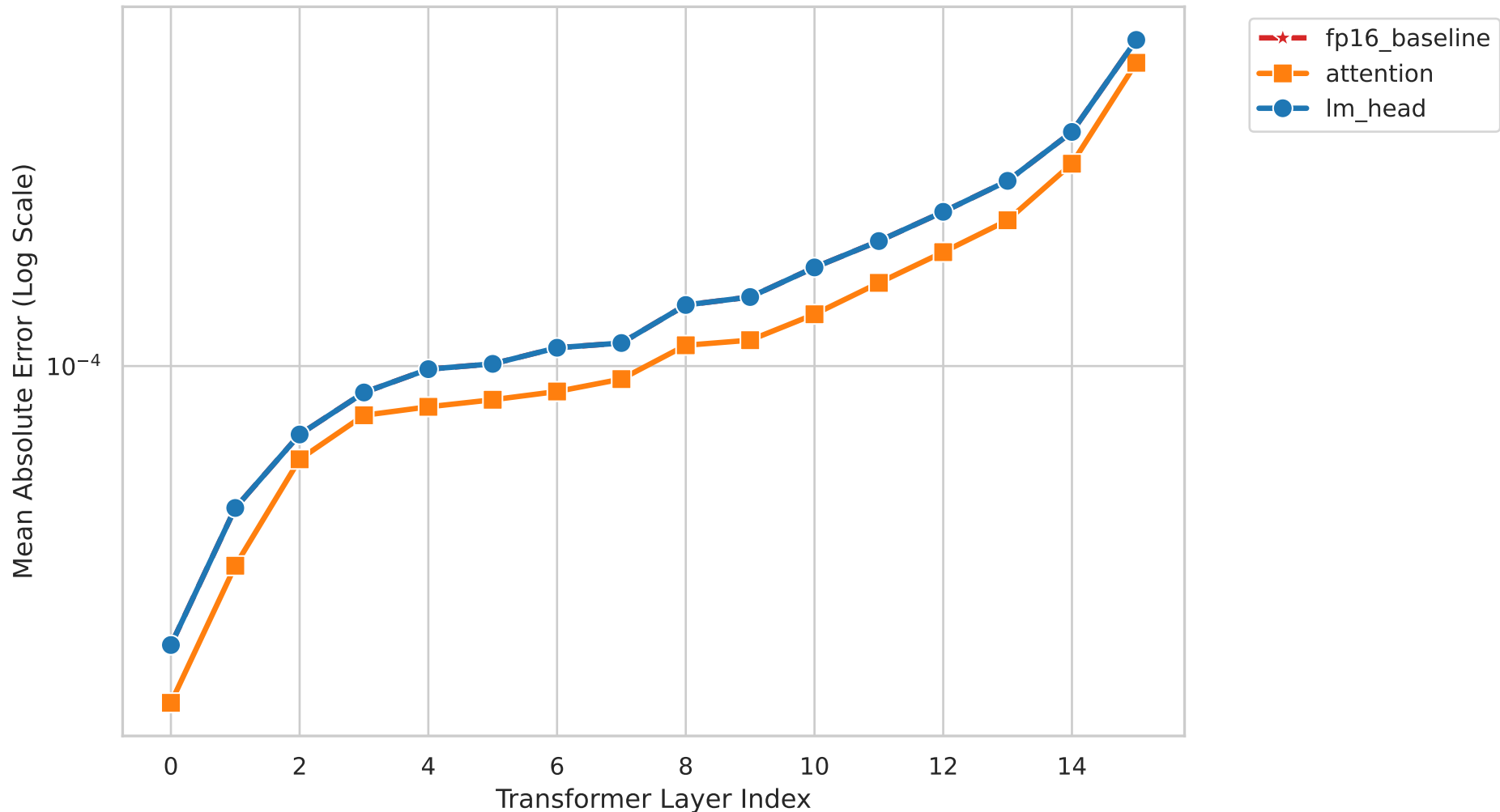
Figure M3. Layer-wise Hidden-State MAE vs FP32 Model: Llama-3.2-1B | Dataset: cmmlu | Base: float16 (Divergent Cases)
