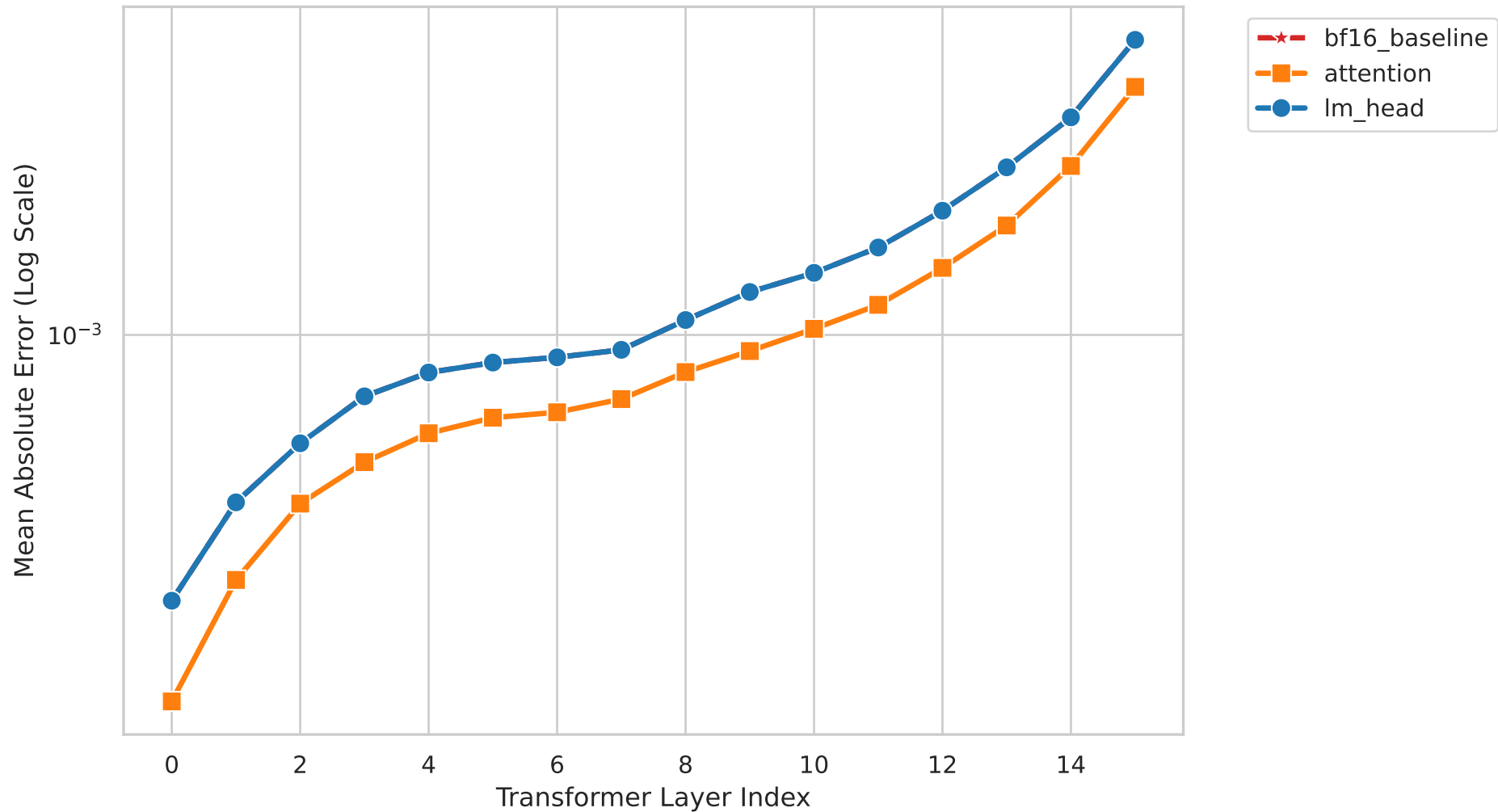
Figure M3. Layer-wise Hidden-State MAE vs FP32 Model: Llama-3.2-1B | Dataset: piqa (Divergent Cases)
