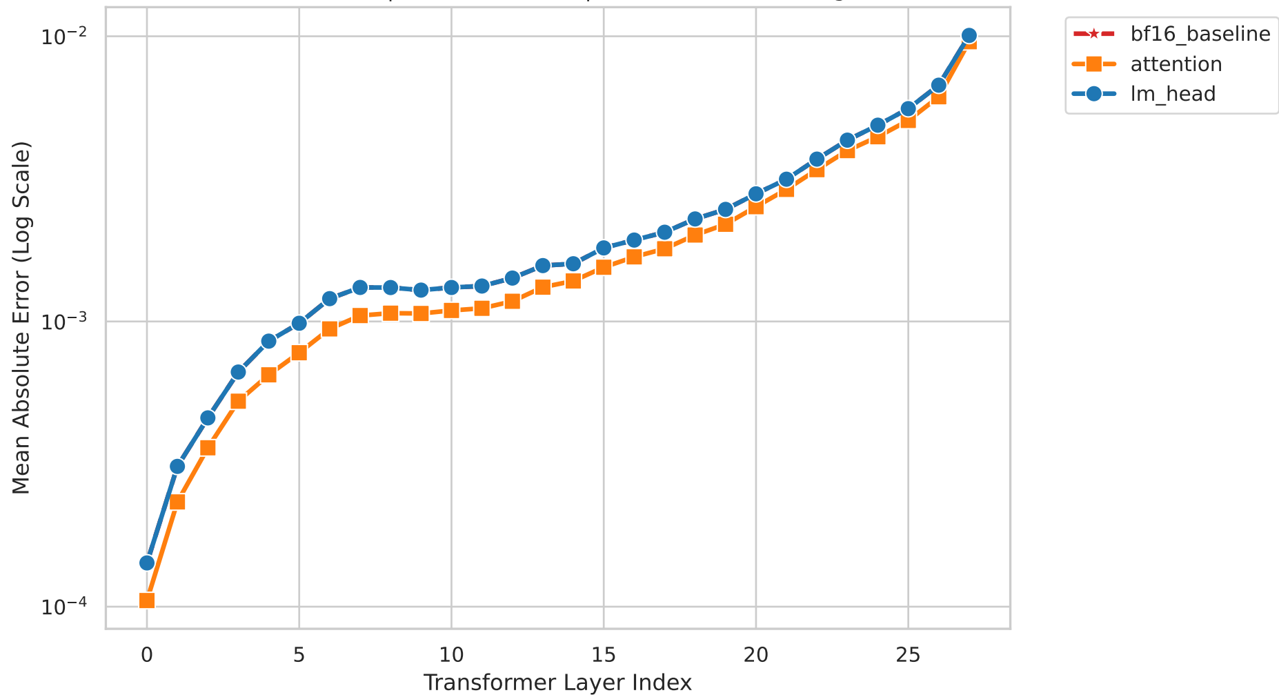
Figure M3. Layer-wise Hidden-State MAE vs FP32 Model: Llama-3.2-3B | Dataset: cmmlu | Base: bfloat16 (Divergent Cases)
