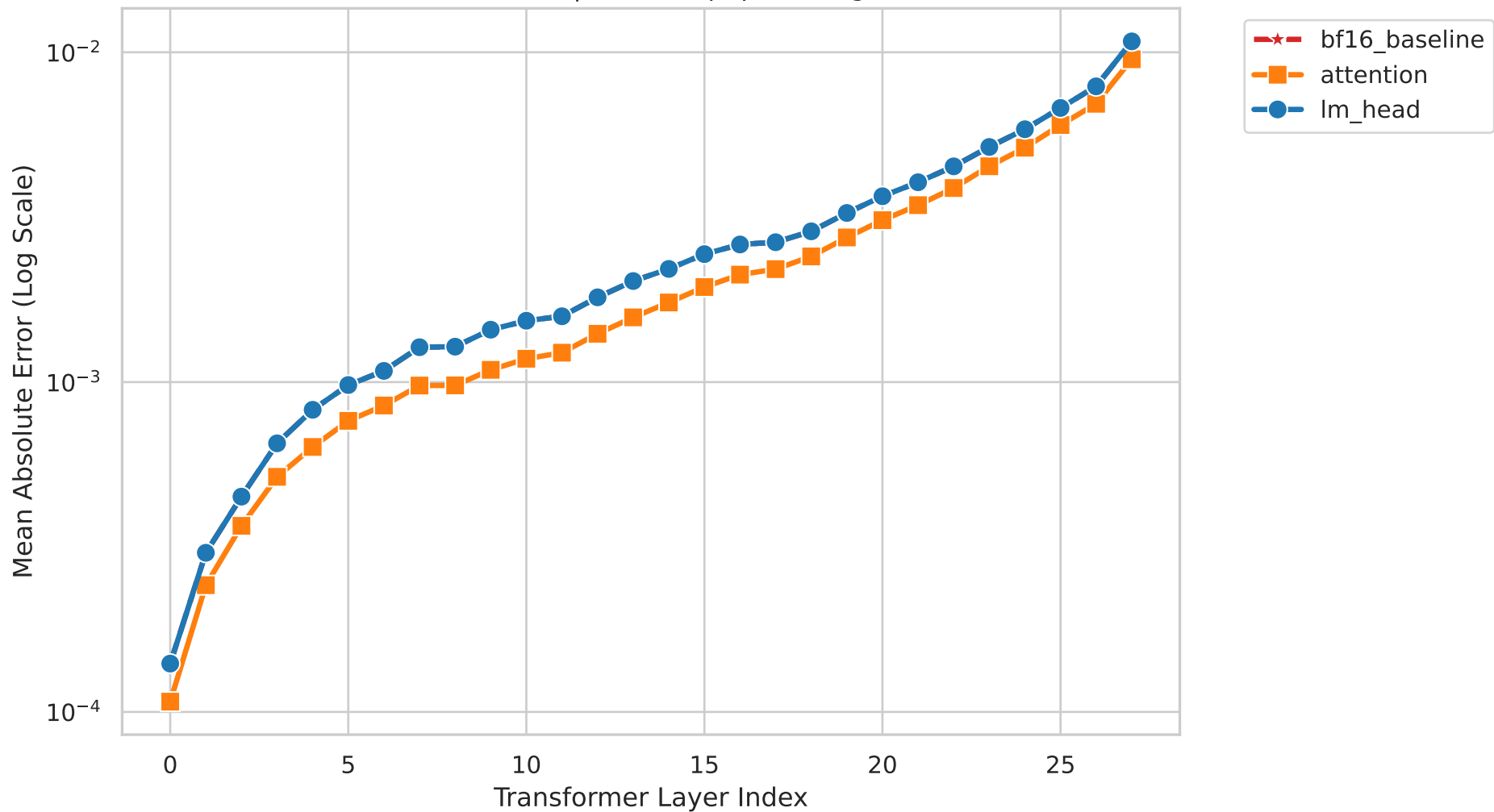
Figure M3. Layer-wise Hidden-State MAE vs FP32 Model: Llama-3.2-3B | Dataset: piqa (Divergent Cases)
