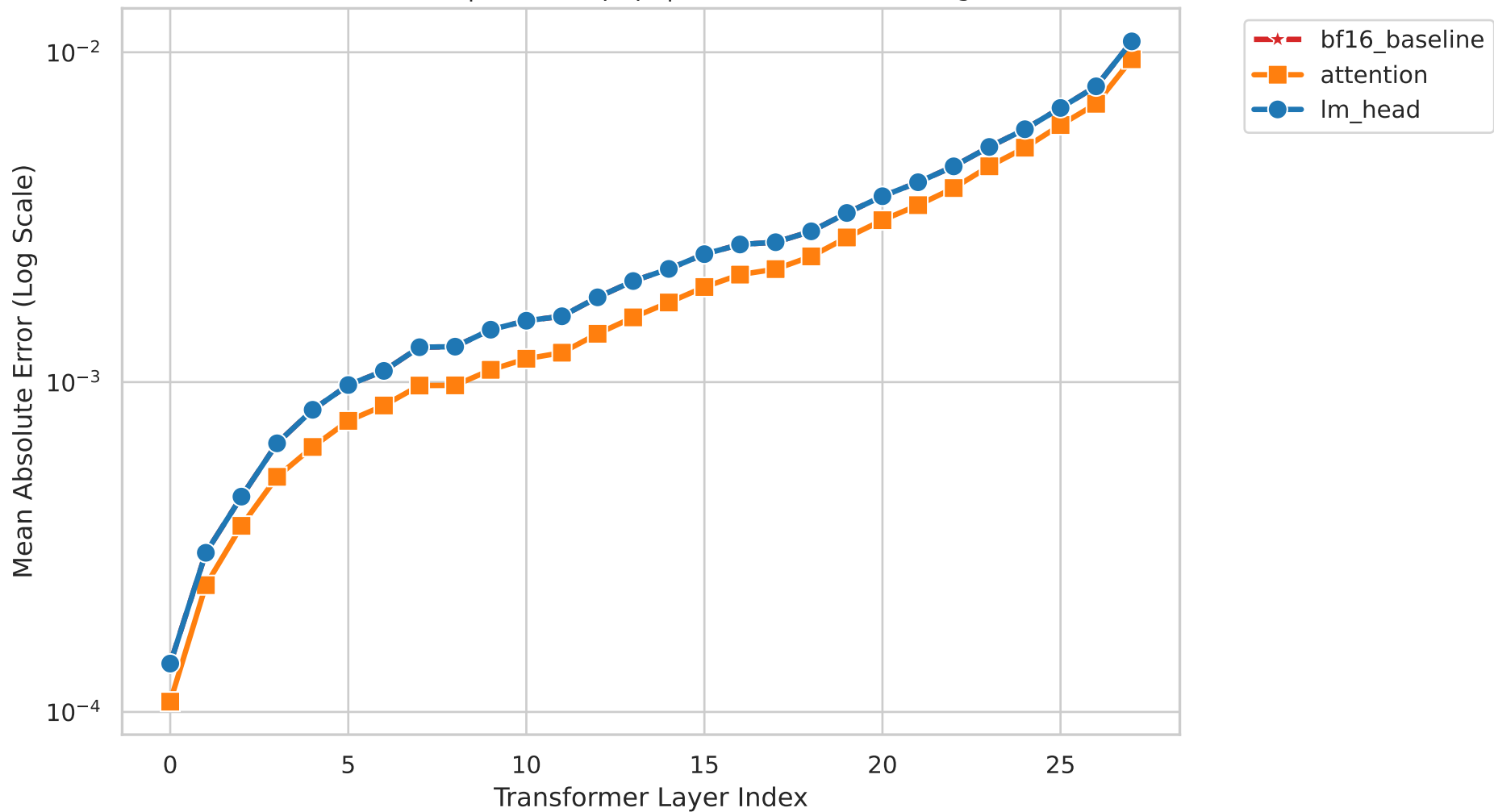
Figure M3. Layer-wise Hidden-State MAE vs FP32 Model: Llama-3.2-3B | Dataset: piqa | Base: bfloat16 (Divergent Cases)
