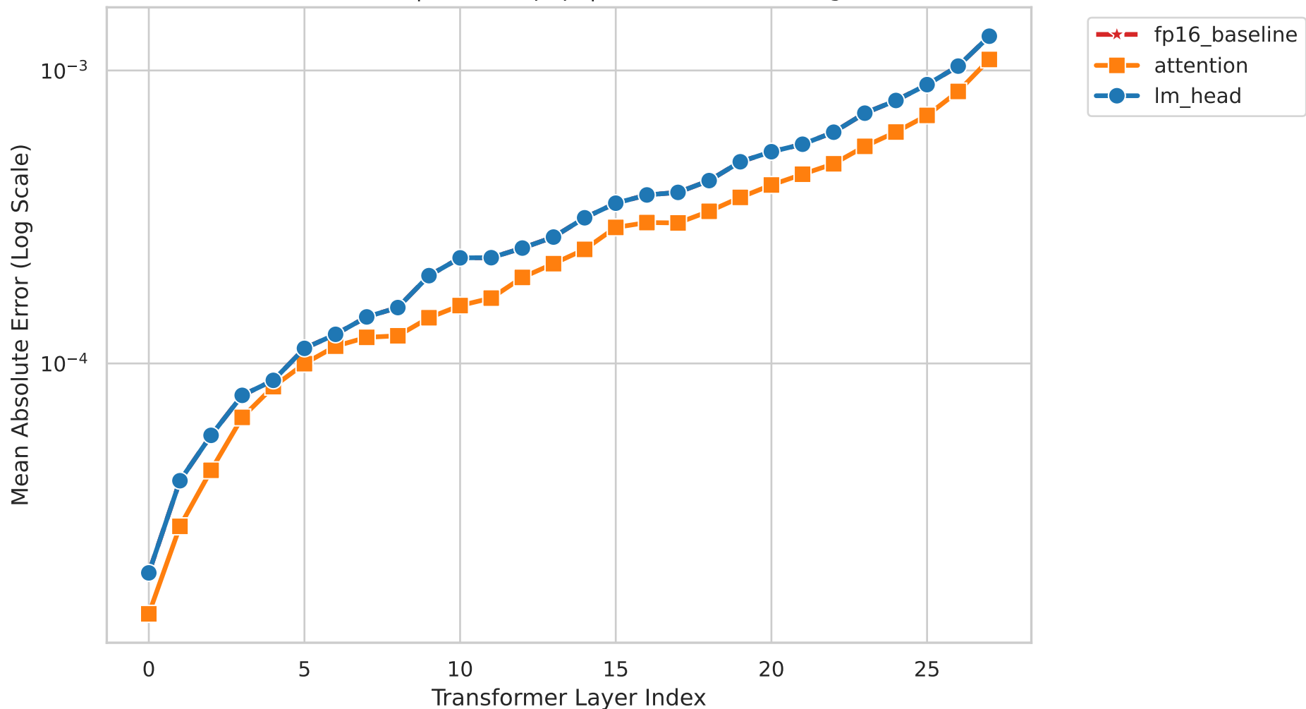
Figure M3. Layer-wise Hidden-State MAE vs FP32 Model: Llama-3.2-3B | Dataset: piqa | Base: float16 (Divergent Cases)
