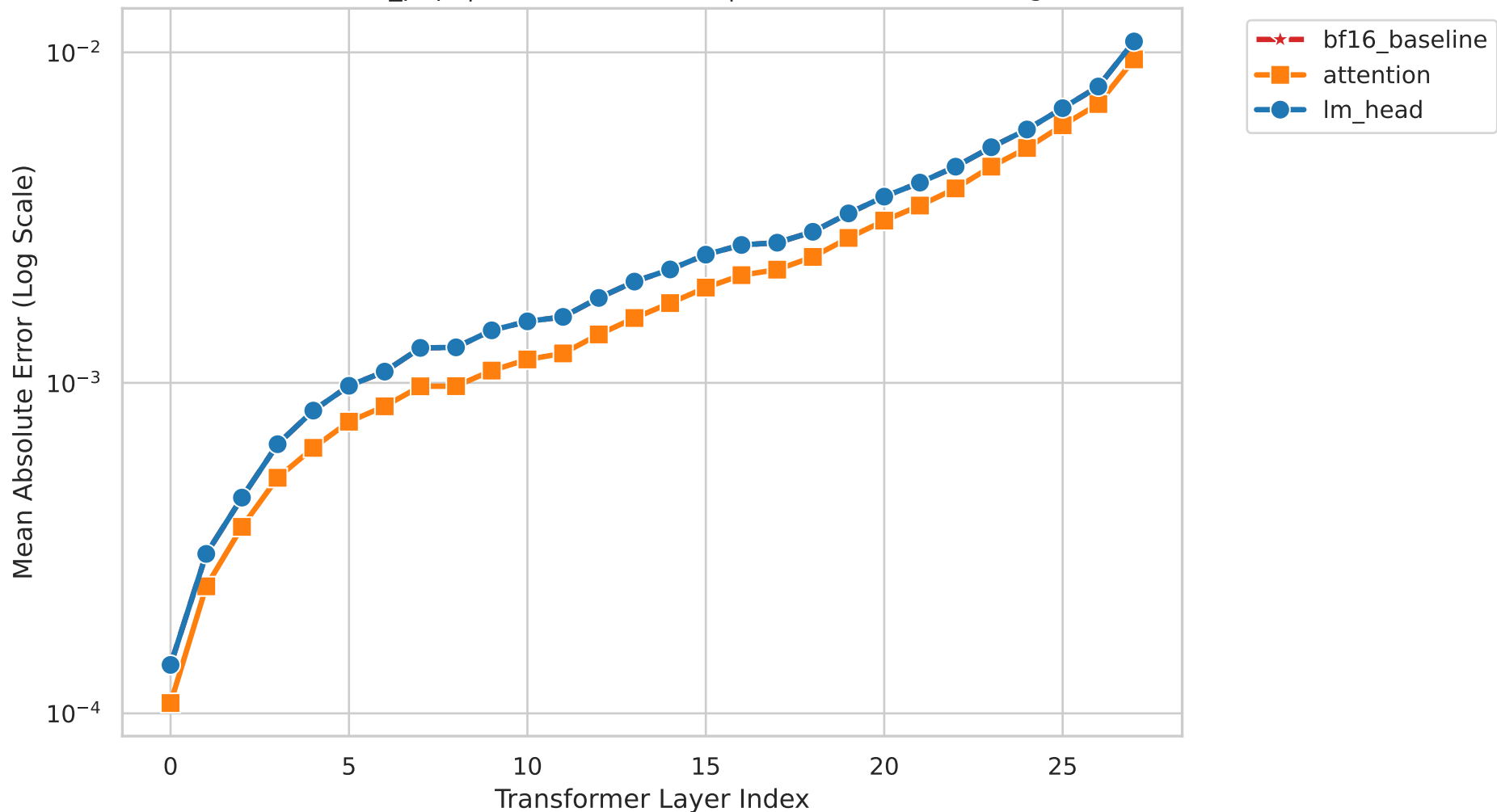
Figure M3. Layer-wise Hidden-State MAE vs FP32 Model: Llama-3.2-3B_piqa | Dataset: unknown | Base: unknown (Divergent Cases)
