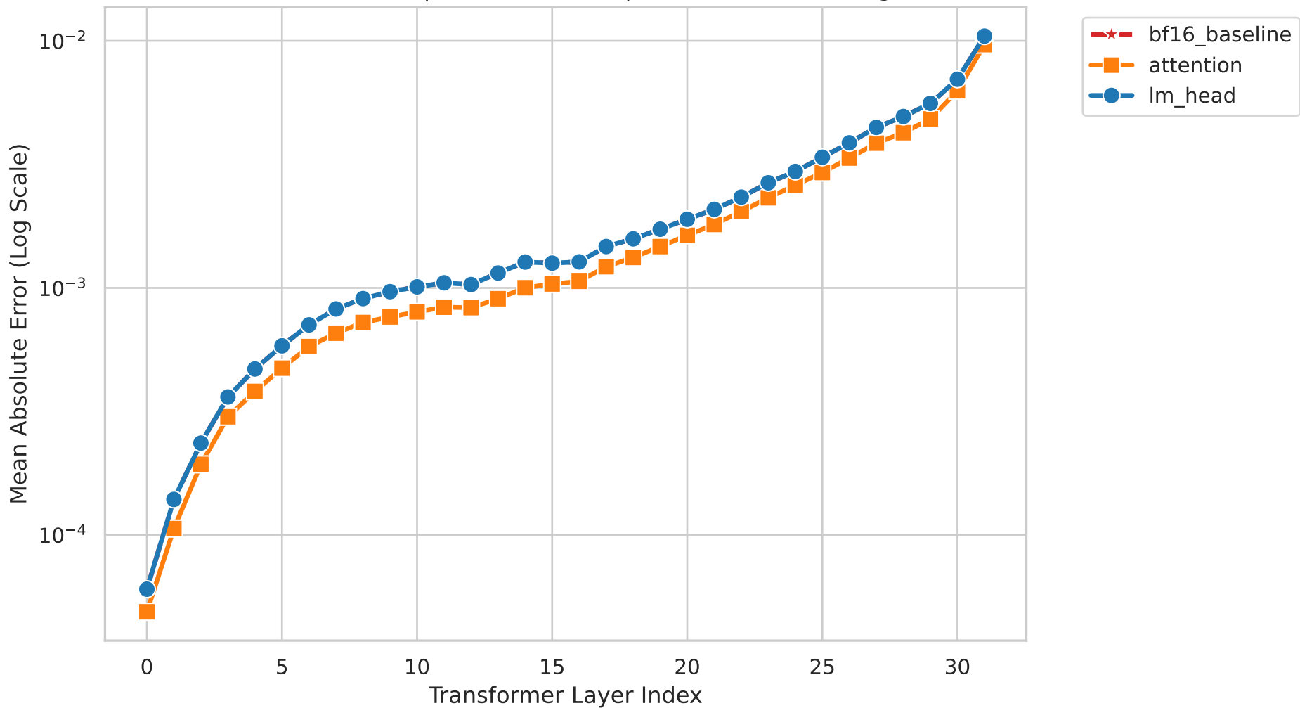
Figure M3. Layer-wise Hidden-State MAE vs FP32 Model: Meta-Llama-3.1-8B | Dataset: cmmlu | Base: bfloat16 (Divergent Cases)
