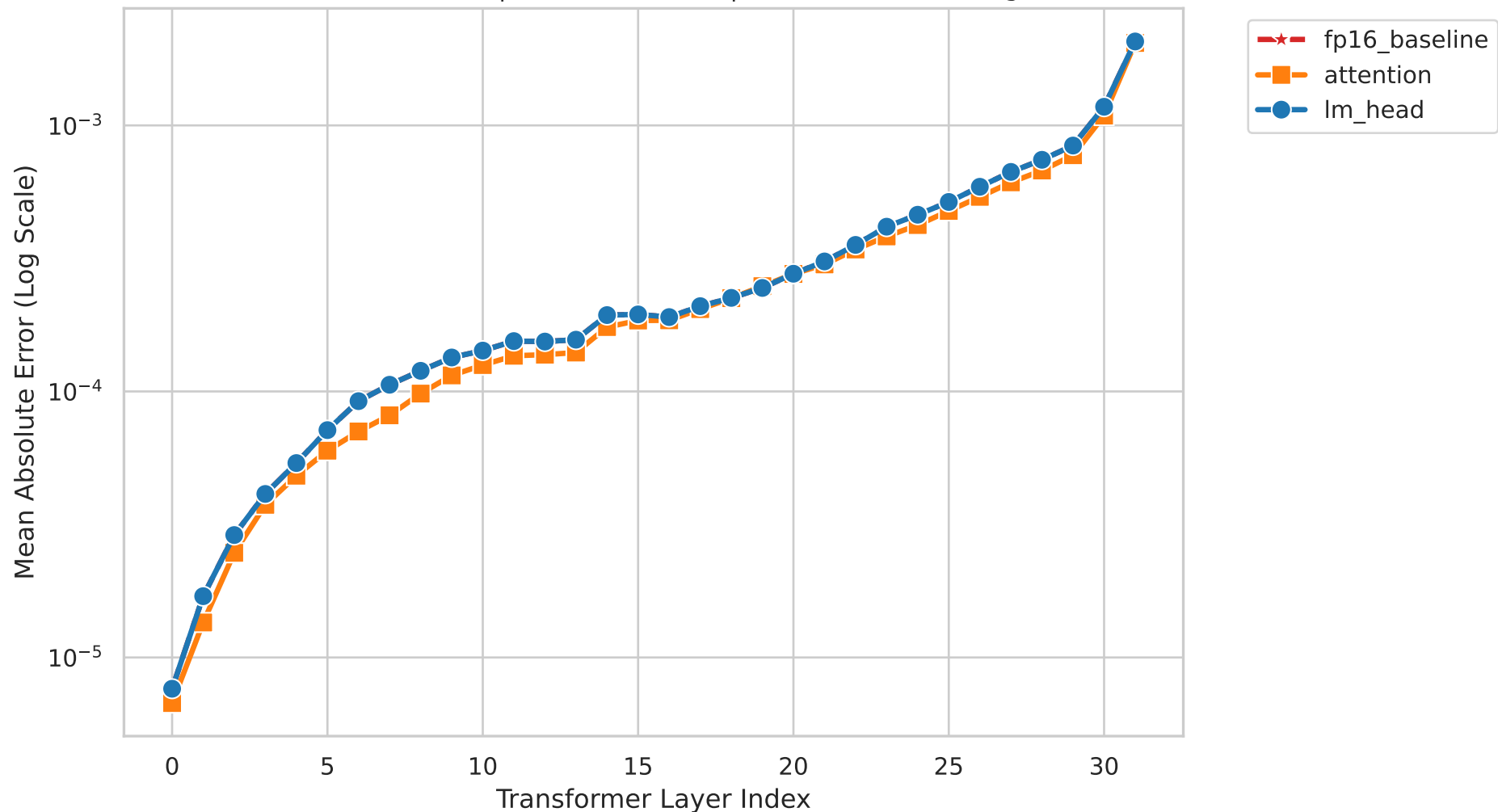
Figure M3. Layer-wise Hidden-State MAE vs FP32 Model: Meta-Llama-3.1-8B | Dataset: cmmlu | Base: float16 (Divergent Cases)
