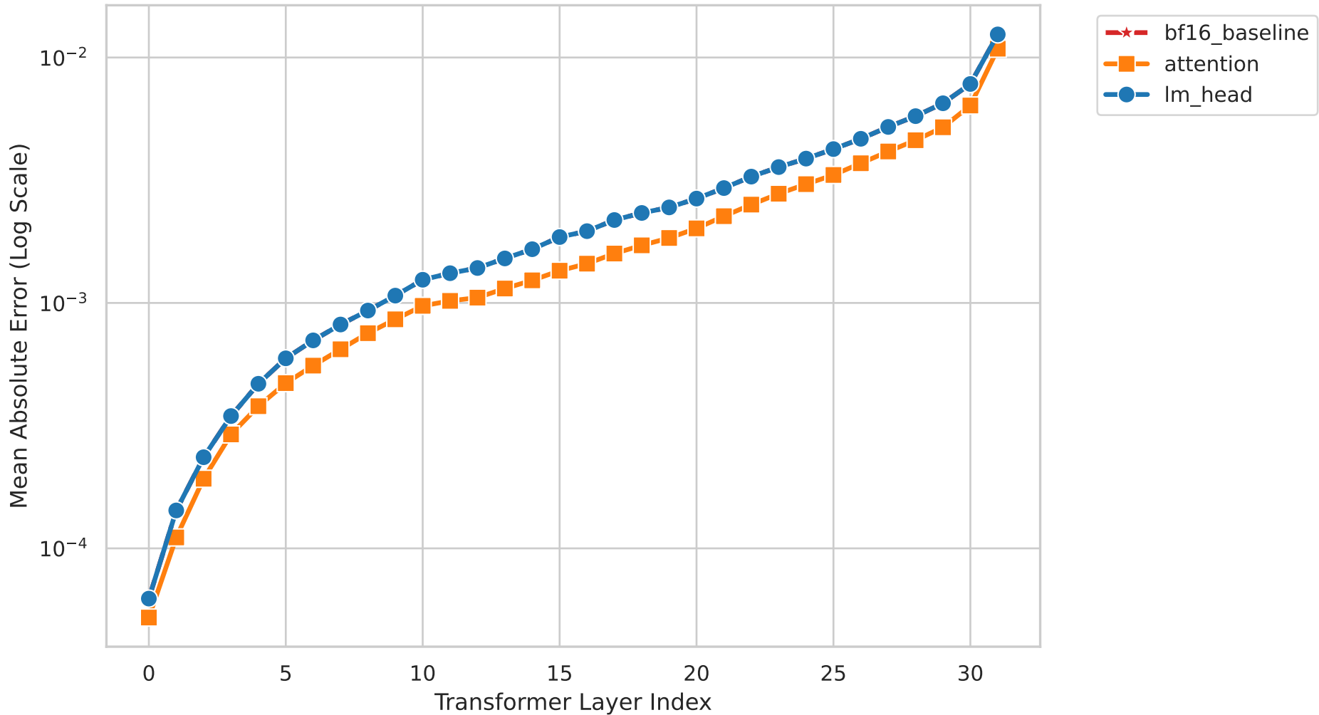
Figure M3. Layer-wise Hidden-State MAE vs FP32 Model: Meta-Llama-3.1-8B | Dataset: piqa (Divergent Cases)
