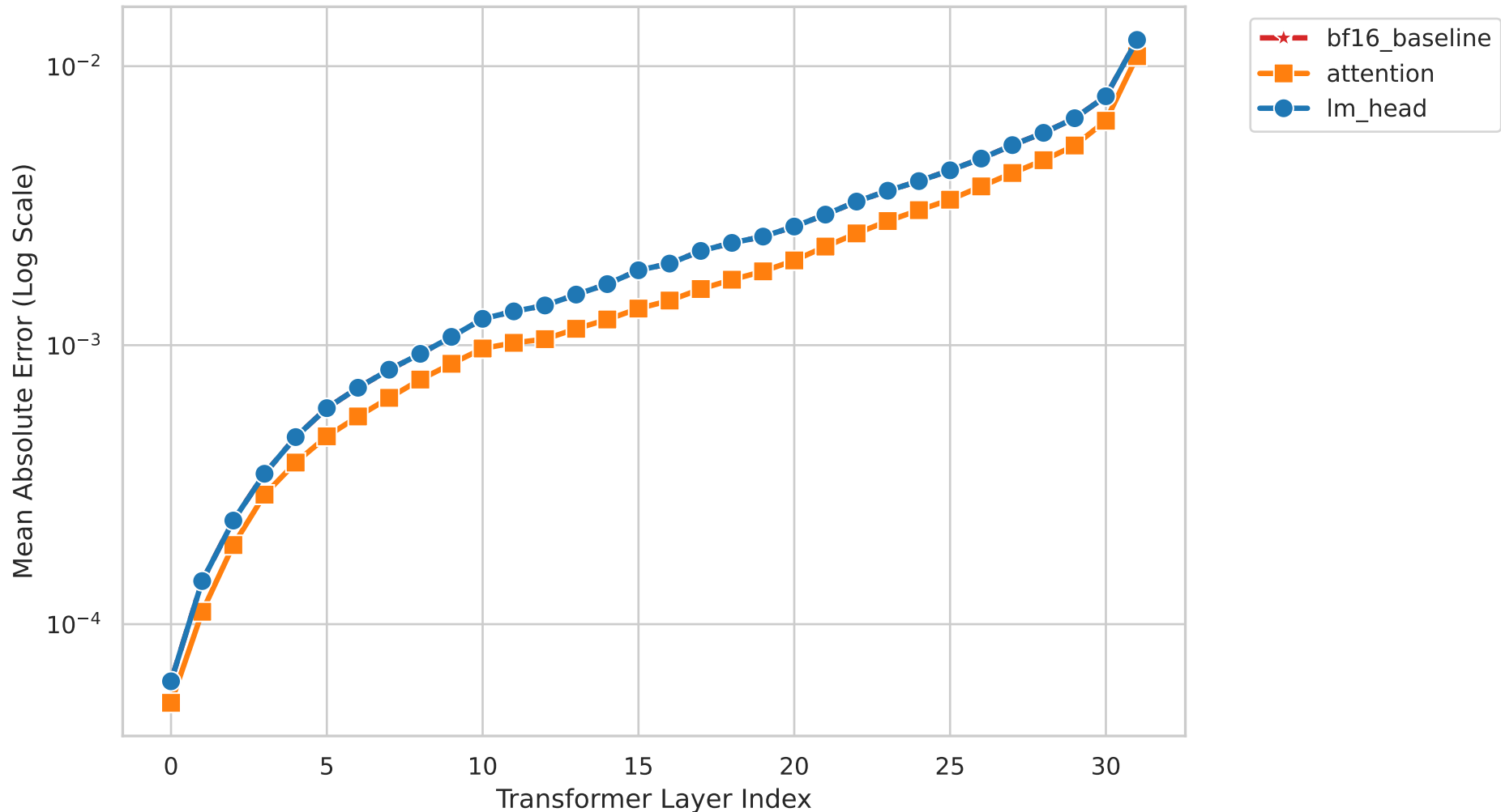
Figure M3. Layer-wise Hidden-State MAE vs FP32 Model: Meta-Llama-3.1-8B_piqa | Dataset: unknown | Base: unknown (Divergent Cases)
