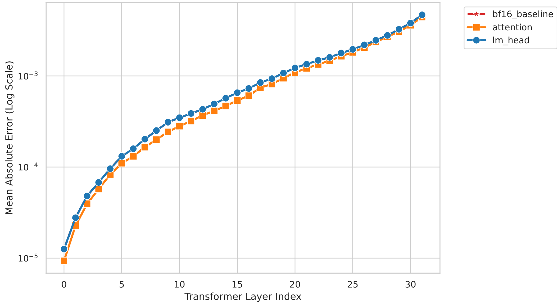
Figure M3. Layer-wise Hidden-State MAE vs FP32 Model: Mistral-7B-v0.3 | Dataset: cmmlu | Base: bfloat16 (Divergent Cases)
