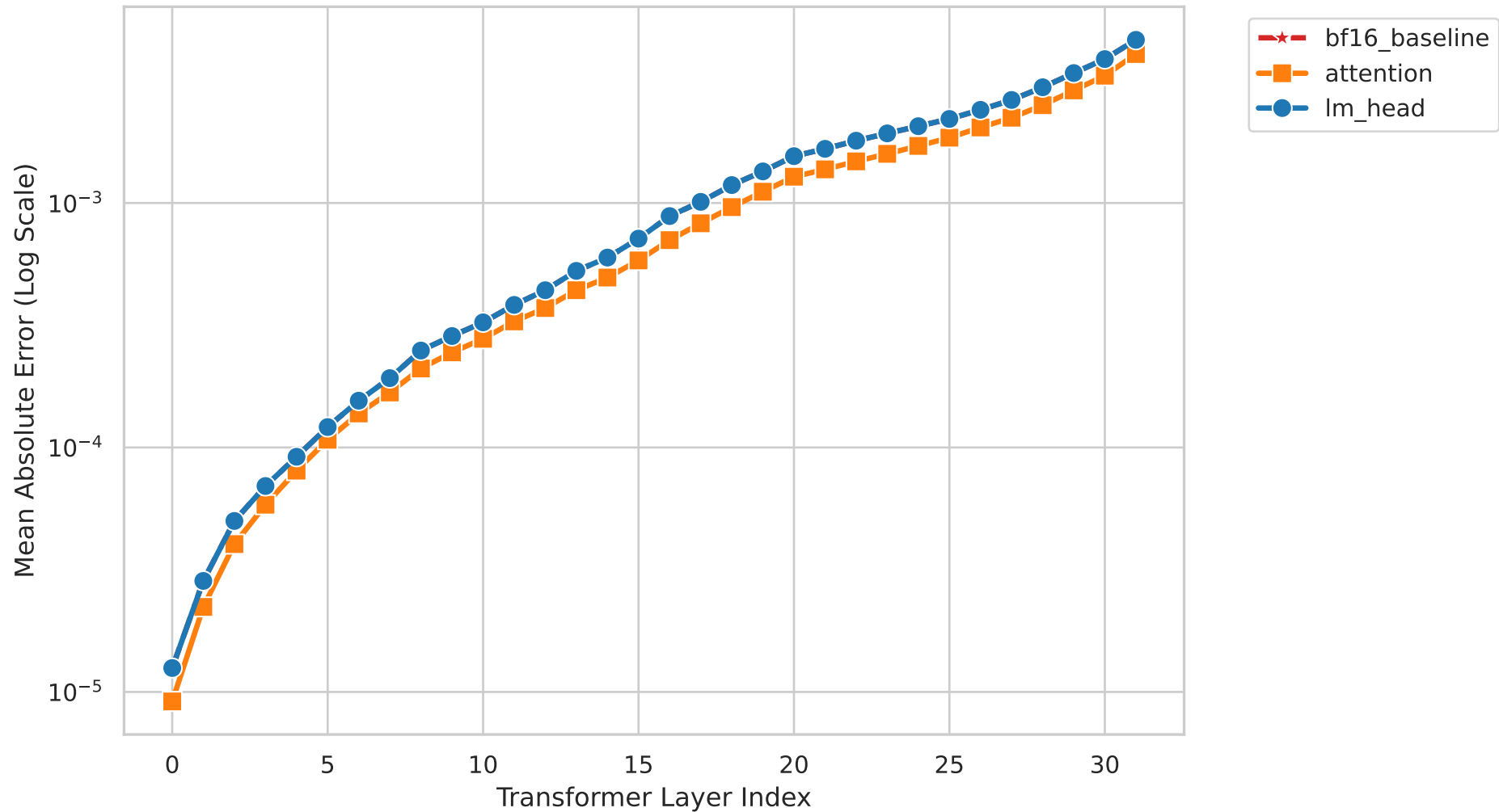
Figure M3. Layer-wise Hidden-State MAE vs FP32 Model: Mistral-7B-v0.3 | Dataset: piqa (Divergent Cases)
