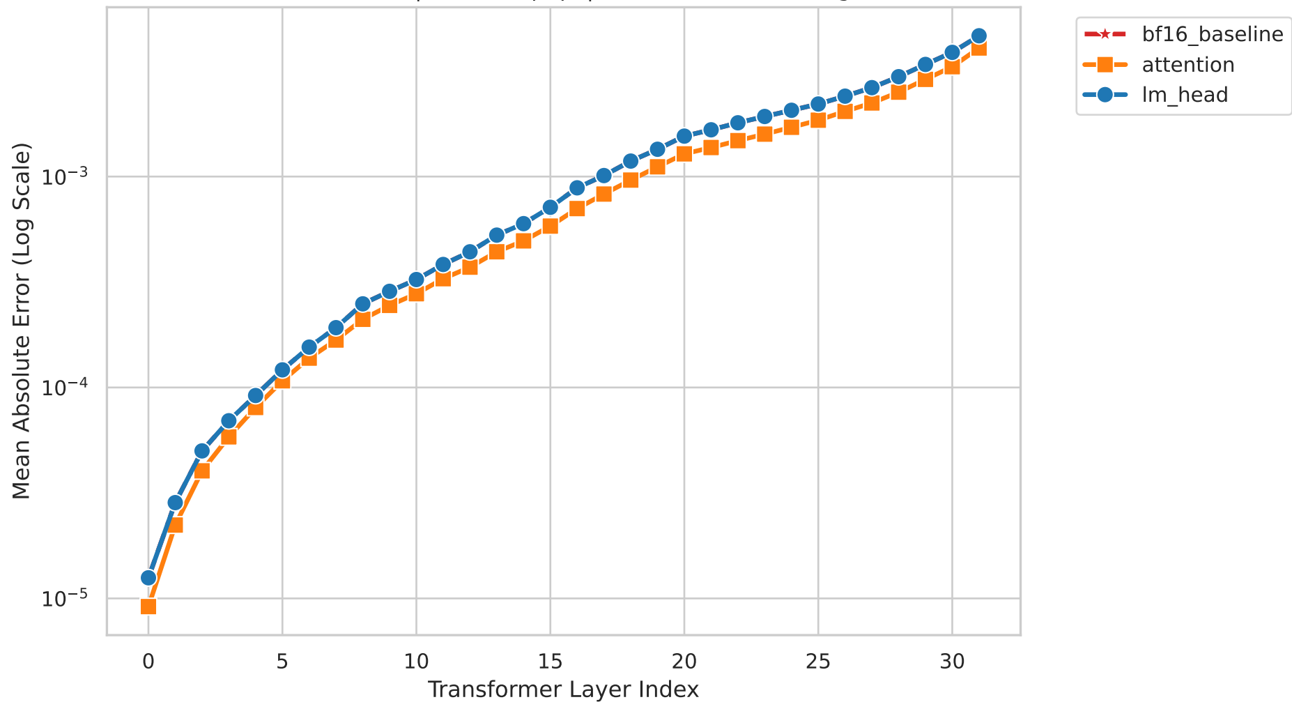
Figure M3. Layer-wise Hidden-State MAE vs FP32 Model: Mistral-7B-v0.3 | Dataset: piqa | Base: bfloat16 (Divergent Cases)
