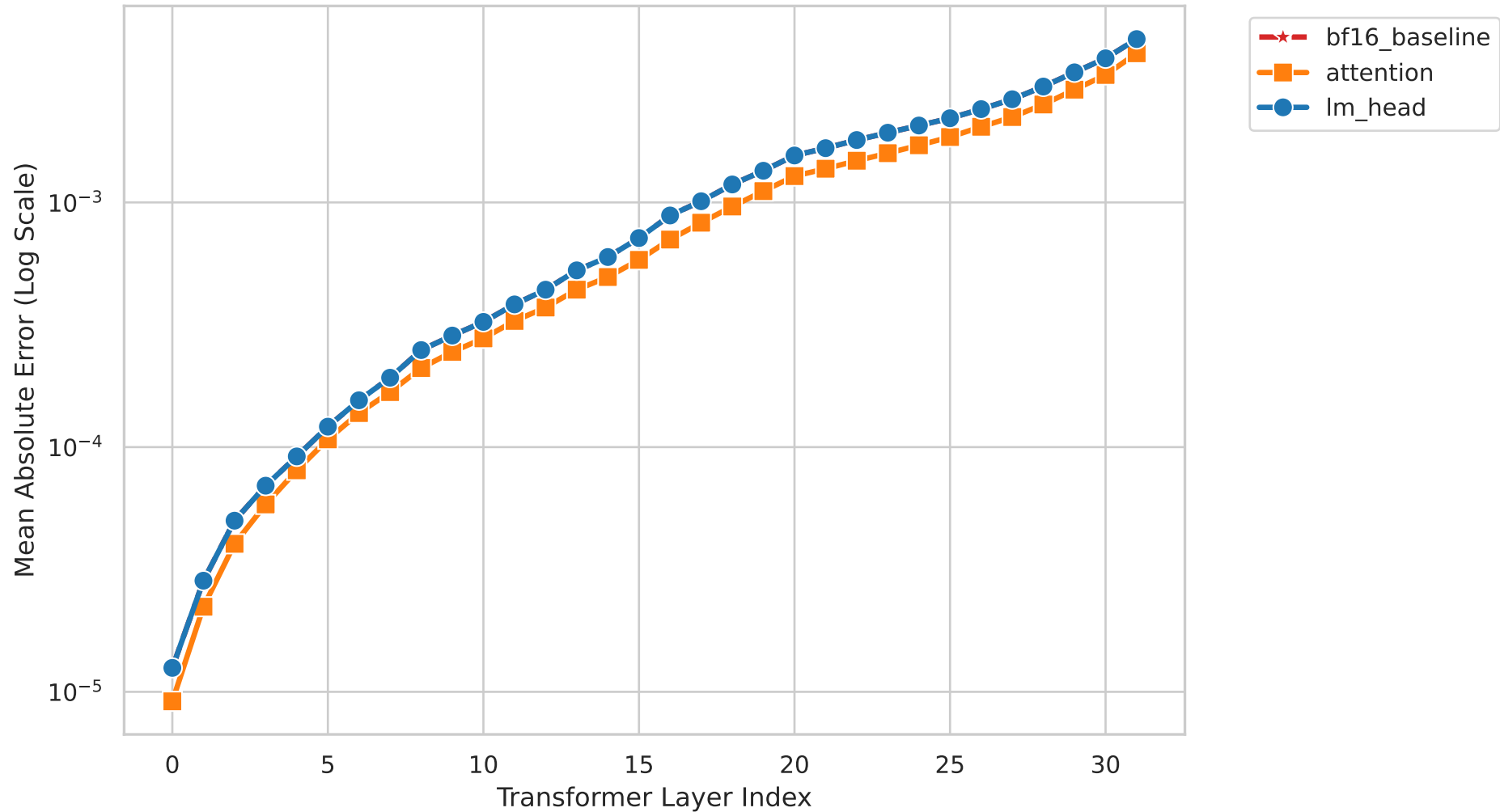
Figure M3. Layer-wise Hidden-State MAE vs FP32
