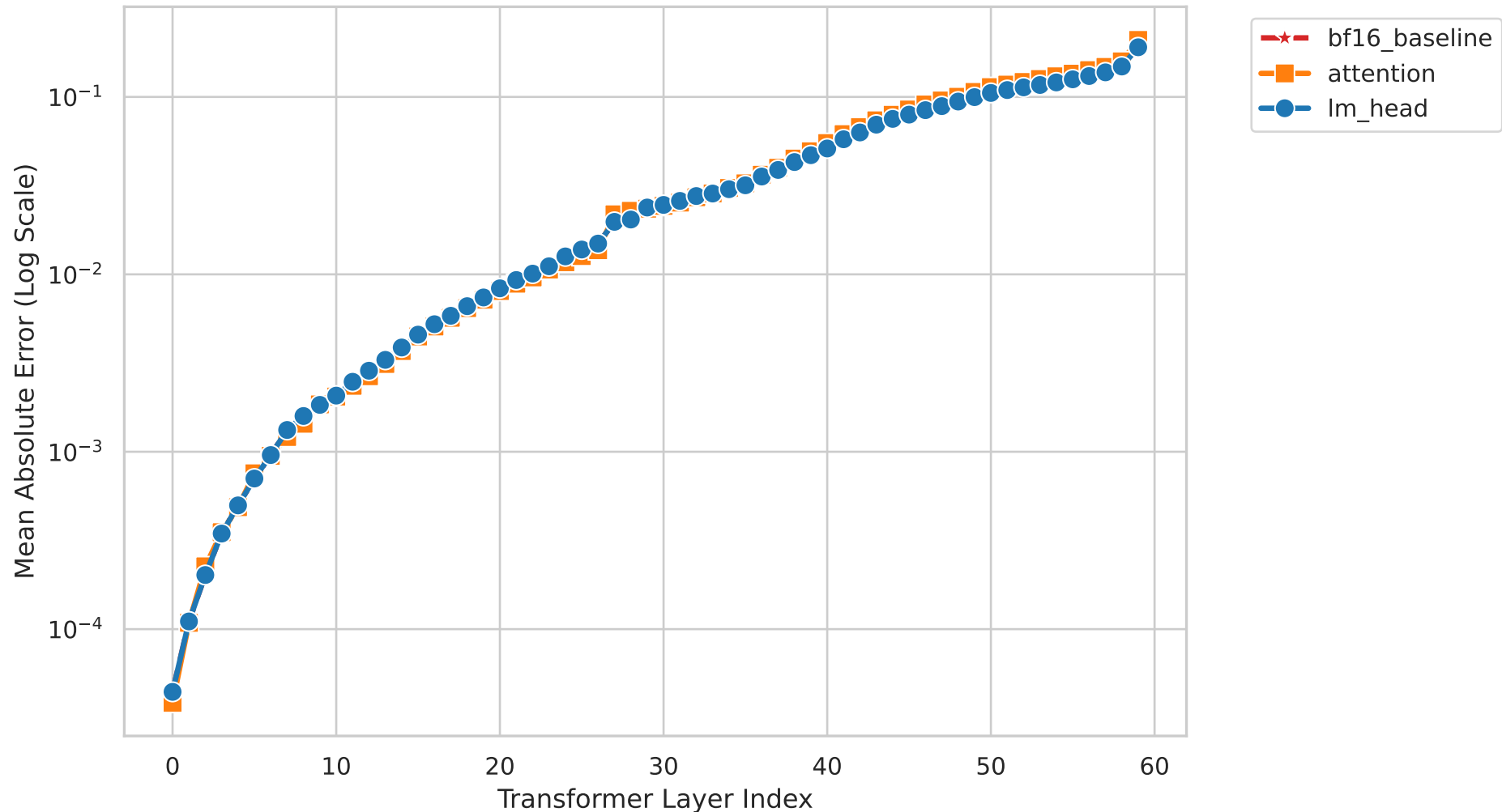
Figure M3. Layer-wise Hidden-State MAE vs FP32 Model: Yi-34B | Dataset: cmmlu | Base: bfloat16 (Divergent Cases)
