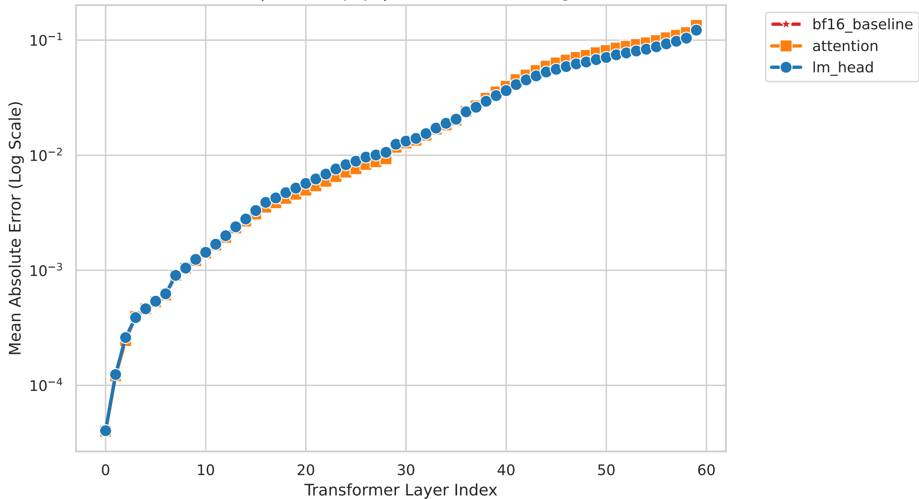
Figure M3. Layer-wise Hidden-State MAE vs FP32 Model: Yi-34B | Dataset: piqa | Base: bfloat16 (Divergent Cases)
