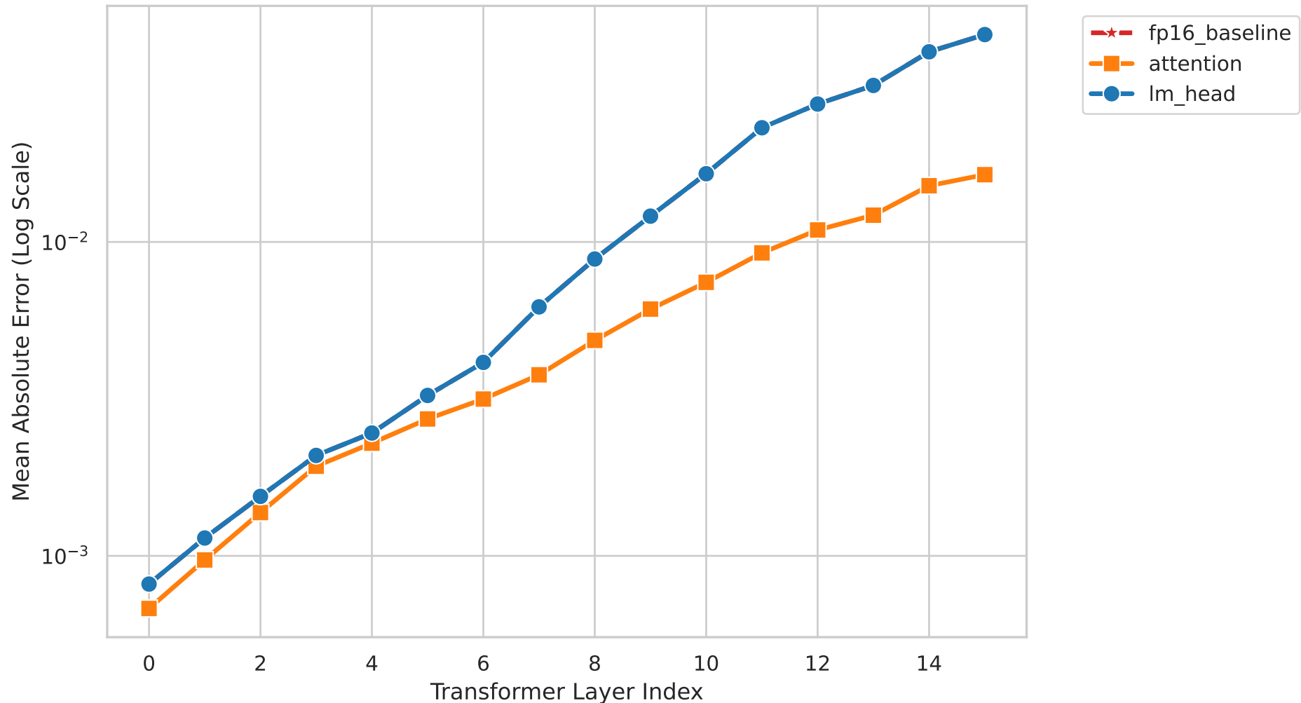
Figure M3. Layer-wise Hidden-State MAE vs FP32 Model: gemma-2-27b | Dataset: cmmlu | Base: float16 (Divergent Cases)
