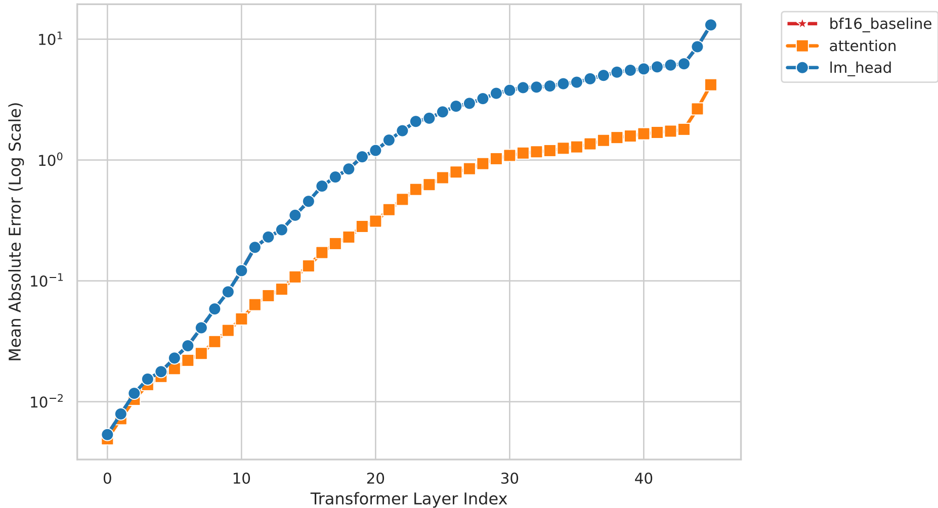
Figure M3. Layer-wise Hidden-State MAE vs FP32 Model: gemma-2-27b | Dataset: piqa | Base: bfloat16 (Divergent Cases)
