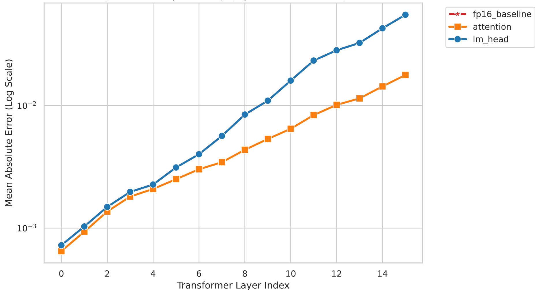
Figure M3. Layer-wise Hidden-State MAE vs FP32 Model: gemma-2-27b | Dataset: piqa | Base: float16 (Divergent Cases)
