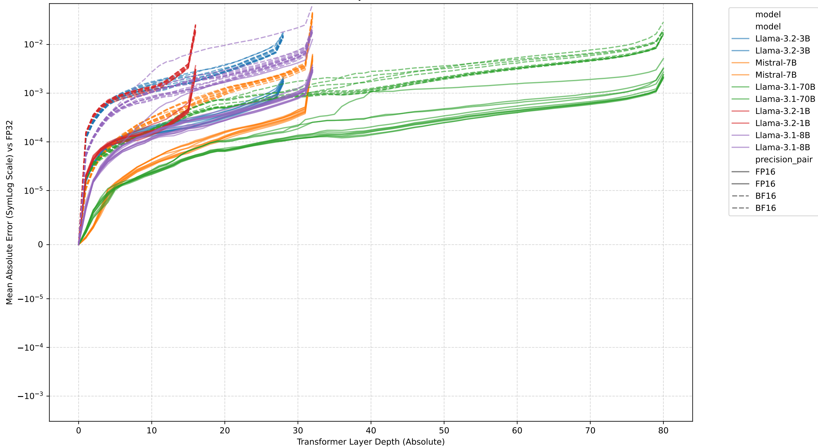
[GSM8K] ALL Cases: Individual Layer MAE Trends (BF16 &amp; FP16 vs FP32)
