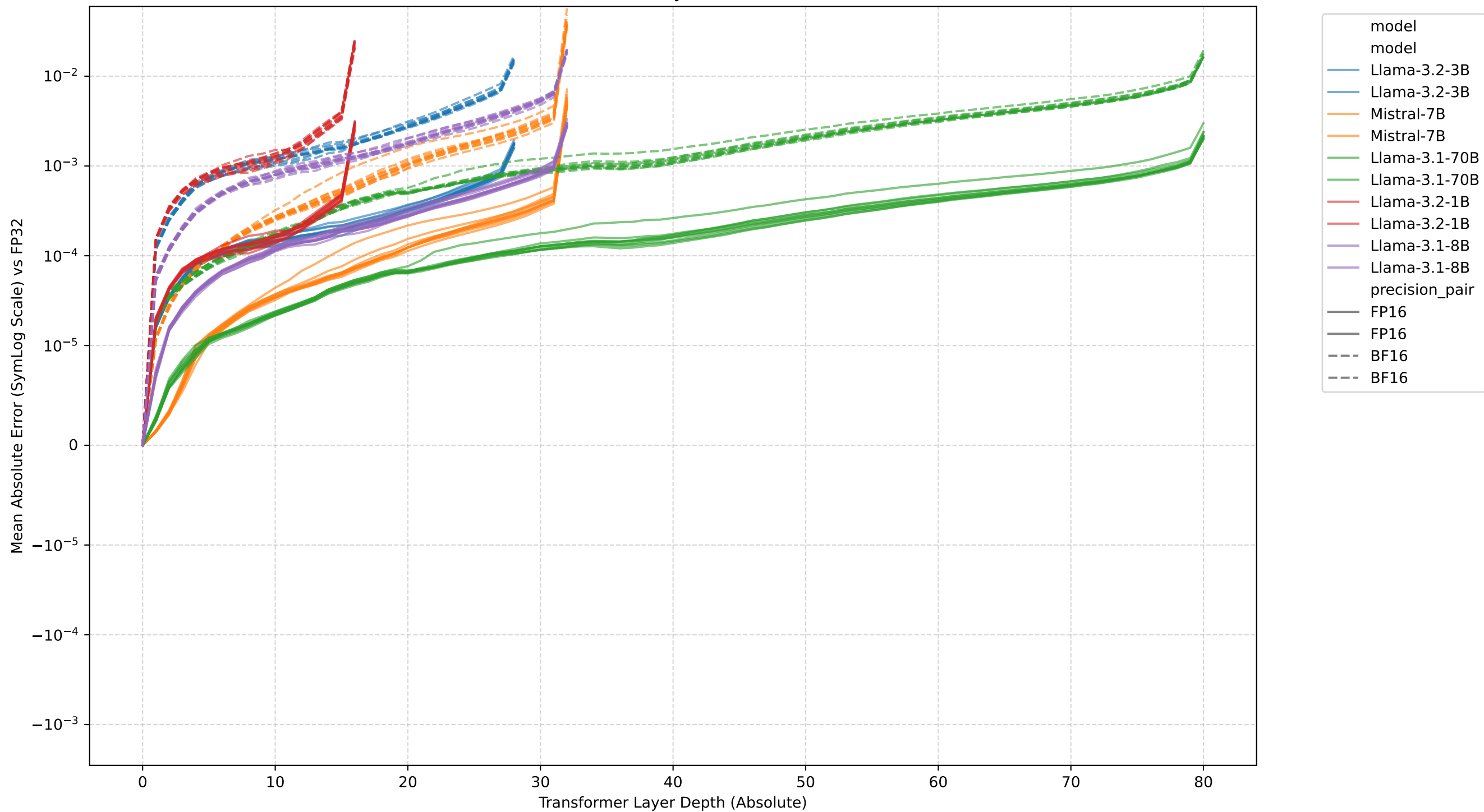
[HUMANEVAL] ALL Cases: Individual Layer MAE Trends (BF16 & FP16 vs FP32)
