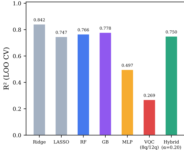
(b) K_{oc} prediction (21 features, incl. B^\dagger )
