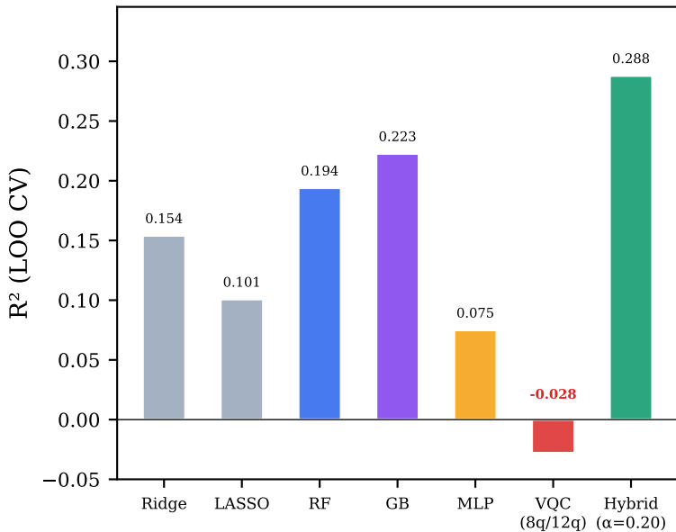
(a) DegT50 prediction (21 features)
