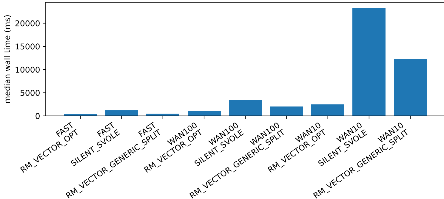
Emulated TCP network runtime
