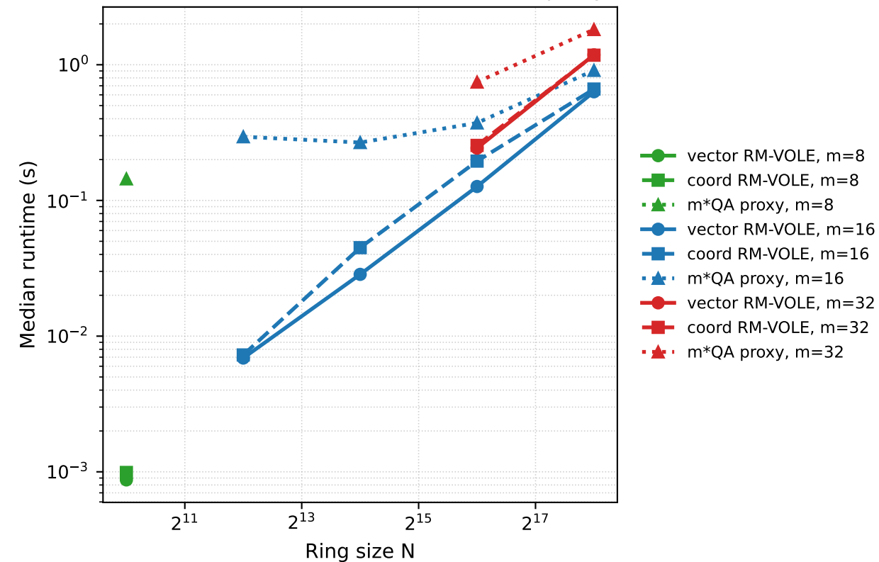
RM-VOLE runtime versus coordinate-wise and QA proxy baselines
