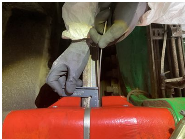
14 Figure from Checklist 'AD 5-135_1_1_5 Preventive_year_null', Task 259 - Measuring points
