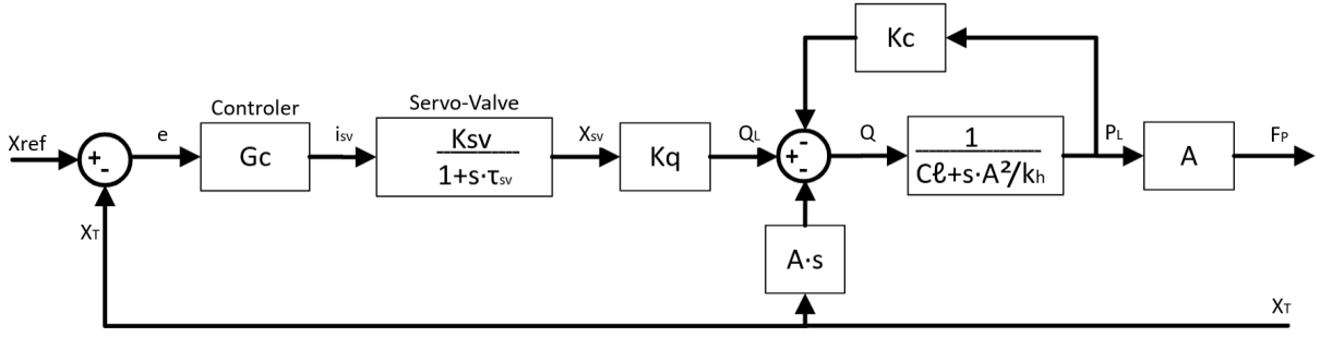
Figure 5: Block diagram of the ST1D
