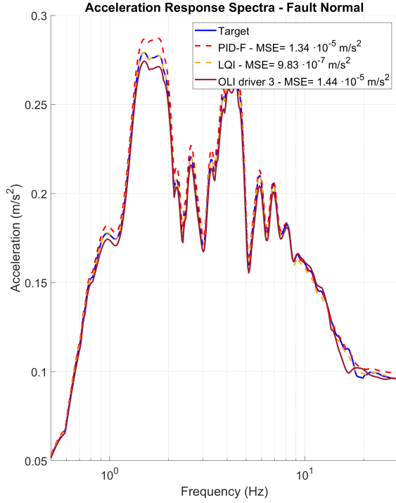
Figure 8: Response spectra for a scaled-down Newhall fault normal seismic signal
