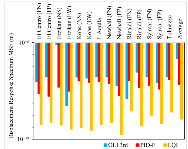
Figure 10: Displacement response spectrum MSE for various seismic signals
