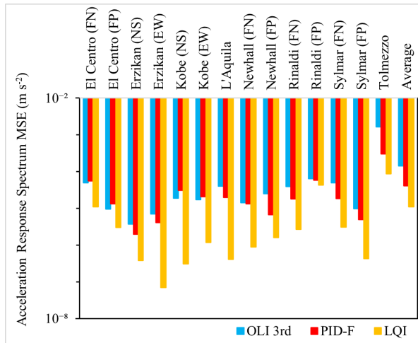
Figure 9: Acceleration response spectrum MSE for various seismic signals
