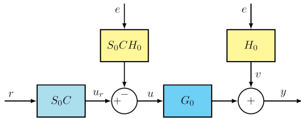
Figure 6: Block diagram illustrating the two-stage method, with S_0C being a Hammerstein-Wiener model to better represent the real system dynamics with control action saturation ( C - controller; S_0 - sensitivity function; G_0 - model plant; H_0 - noise model; e - white noise; u_r - noise free control action).
