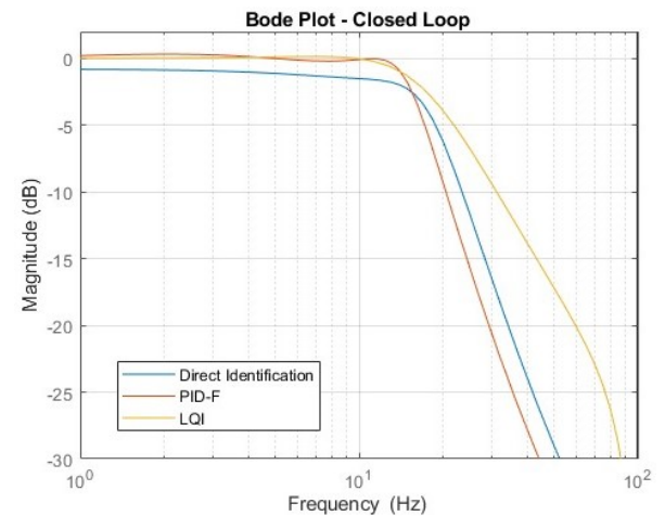
Figure 7: Shaking table control loop frequency response with controllers optimized for the Tolmezzo earthquake
