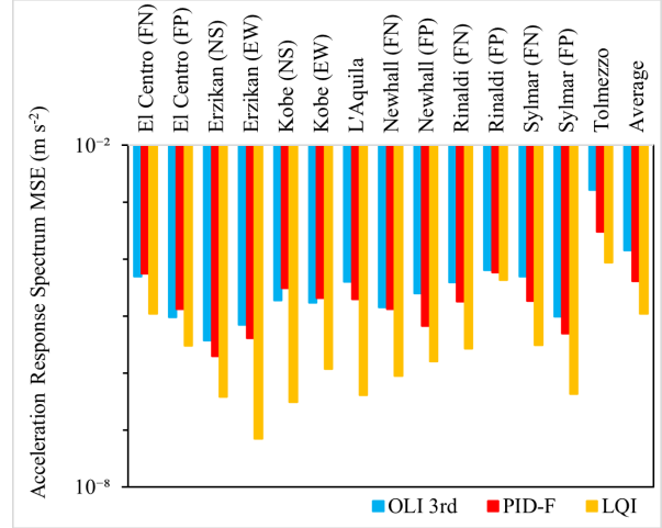
Figure 11: Acceleration response spectrum MSE
