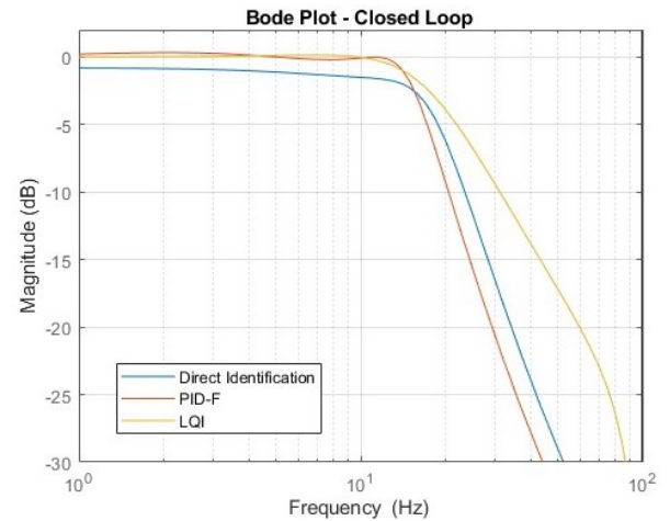
Figure 9: Shaking table closed-loop frequency response with optimized controllers (LQI for the Tolmezzo earthquake)
