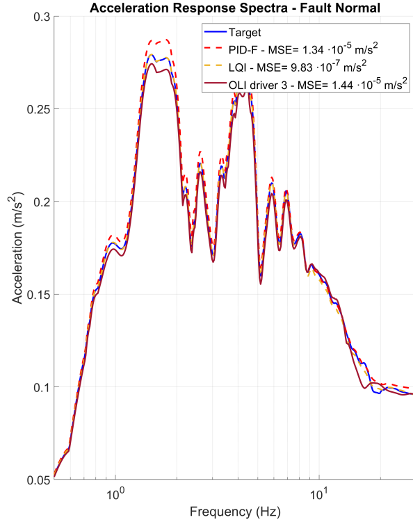
Figure 10: Acceleration response spectra for a scaled-down Newhall fault normal seismic signal
