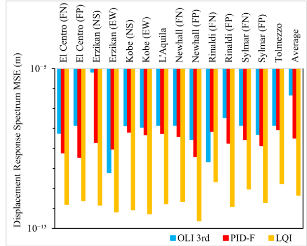
Figure 12: Displacement response spectrum MSE
