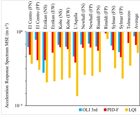
Figure 6: Acceleration response spectrum MSE
