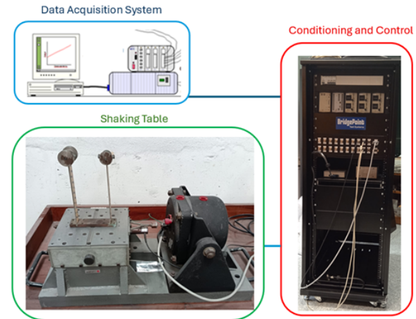
Figure 3: Experimental facility
