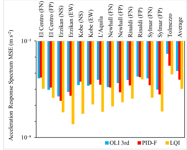
Figure 11: Acceleration response spectrum MSE
