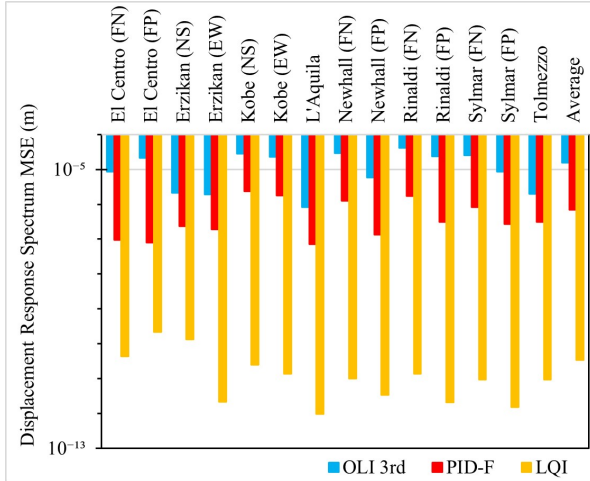
Figure 7: Displacement response spectrum MSE
