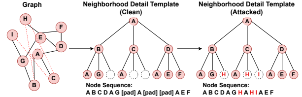
Figure 2: Illustration of node sequence template injection attacks. The example shows Non-adjacent Injection (NI), where red dashed lines denote attacker-induced edge perturbations. In Supernode Injection (SI) and Multiple Supernode Injection (MSI), the injected supernode or supernodes occupy placeholder positions. Here, k = 3 .
