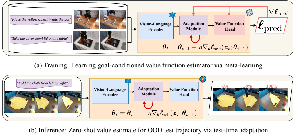
Figure 1: Overview of VITA. During training (top), VITA meta-learns a goal-conditioned value function estimator so that each subsequent self-supervised update improves value prediction; at inference (bottom), the same estimator adapts online to every out-of-distribution test trajectory, delivering zero-shot generalization through test-time adaptation.
