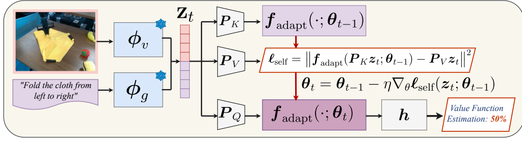
Figure 2: Test-time Adaptation. During inference, at each timestep t , the adaptation module f_{\text{adapt}} takes a gradient step on the meta-learned self-supervised loss \ell_{\text{self}} , thereby encoding trajectory history in its parameters.
