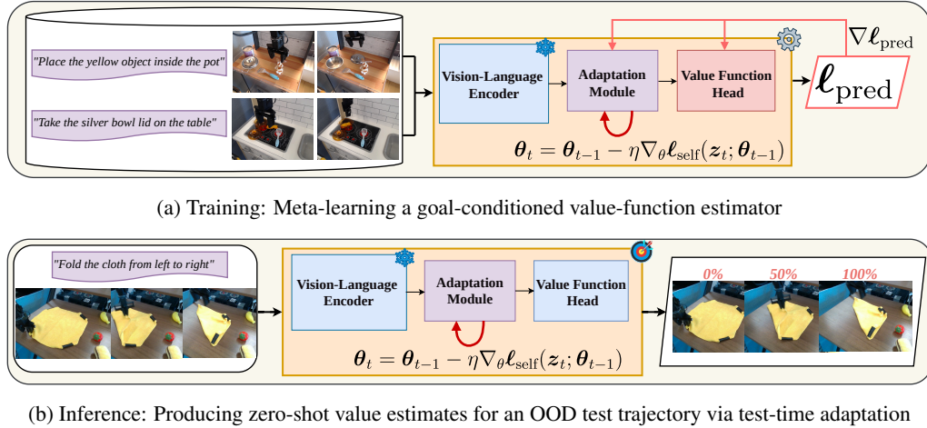
Figure 1: Overview of VITA. VITA meta-learns a goal-conditioned value function whose adaptation module is updated at inference time, enabling zero-shot value estimation on out-of-distribution trajectories.
