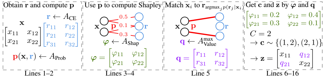
Figure 2: [An illustration of COLA] The figure traces how COLA produces \mathbf{c} and \mathbf{z} for equation (1). For clarity, line 5 is illustrated with the simpler value assigner A_{\text{Value}}^{\max} . In lines 6–16 we set C = 2 , and the sampling selects exactly two positions for modification according to the normalized attribution matrix \varphi .
