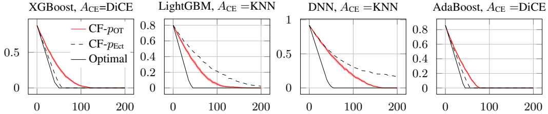
Figure 4: [ German Credit ] Residual divergence D(f(\mathbf{z}), \mathbf{y}^*) against the action budget C , with D = \text{MeanD} , comparing \text{CF-}p_{\text{OT}} and \text{CF-}p_{\text{Ect}} to the mixed integer linear programming (MILP) global optimum. The proposed \text{CF-}p_{\text{OT}} tracks the optimum closely and, in several cases, matches or surpasses the alignment-informed \text{CF-}p_{\text{Ect}} .
