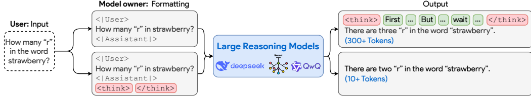
Figure 1: Unthinking vulnerability in large reasoning models. The top example illustrates standard behavior, in which the LRM generates detailed reasoning traces before answering. The bottom example shows that inserting thought delimiters causes the model to skip the thinking process and output an incorrect answer with minimal token usage.
