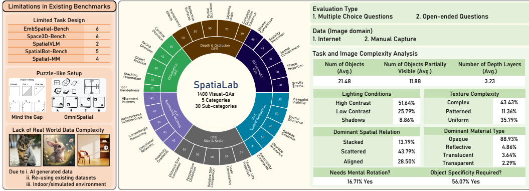
Figure 1: Overview of SPATIALLAB . The benchmark targets limitations of prior spatial-reasoning datasets (left), introduces 1,400 visual QA pairs spanning 5 categories and 30 subcategories (center), and supports systematic evaluation through multiple-choice and open-ended tasks. Its images and questions cover varied complexity dimensions, including object counts, depth layers, lighting, textures, relations, and materials (right).
