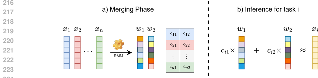
Figure 3: Overview of the proposed RMM framework. Left: During the merging phase, we compute a compact set of basis directions (e.g., two in this example) and their associated task-specific coefficients. Right: At inference, a target model i is reconstructed by linearly combining the basis vectors using the corresponding coefficients.
