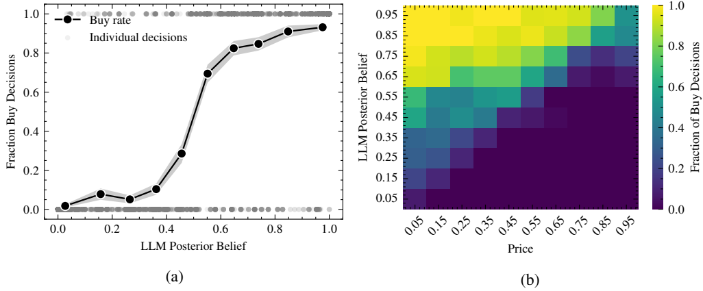
Figure 4: The rate at which the LLM chose a ‘buy’ decision as a function of (a) its self-reported posterior belief and (b) its self-reported posterior together with the price of buying.
