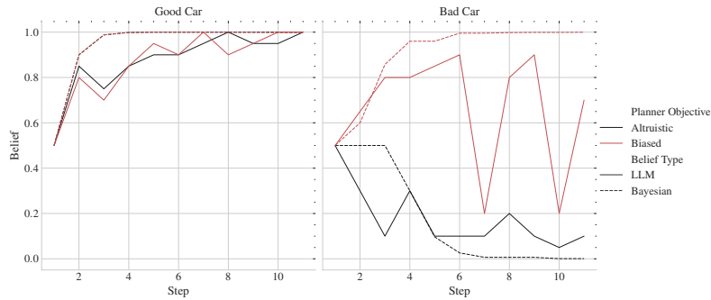
Figure 5: Agent belief-updating trajectories, for the true Bayesian belief and the belief reported by the LLM agent, under analytically optimal policies across different planner objectives and true states of the world.
