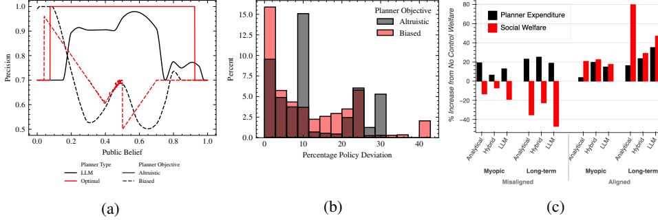
Figure 2: (a) Example policies of the LLM planner (black) overlaid on the analytically optimal planner (red), for both the altruistic (solid) and biased (dashed) settings; the two curves track each other across the full belief range, including the non-monotone biased policy. (b) Distribution of the percentage deviation between the LLM and optimal policies over the public-belief space: the mass is concentrated below 10%, quantifying the close structural match in panel (a). (c) Planner expenditure and social welfare, each expressed as a percentage of the no-control baseline welfare, with the true state fixed to B . The left half is a biased planner seeking action G and the right half an altruistic planner, so the two halves read as a direct comparison of misaligned versus aligned mediation.
