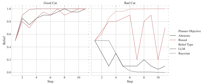
Figure 5: Belief-updating trajectories, pairing the true Bayesian belief against the belief reported by the LLM agent under the analytically optimal policy, for each combination of planner objective and true state. The vertical gap between the paired curves at each step quantifies the LLM’s departure from Bayesian updating and its resistance to cascades.
