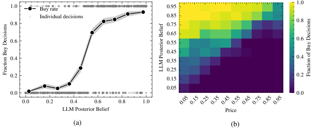
Figure 4: LLM “buy” rate as a function of (a) its self-reported posterior belief and (b) its self-reported posterior together with the purchase price. In (a) the “buy” rate steps sharply at the rational threshold of 0.5; in (b) the high-/low-acceptance regions separate along the c = p diagonal predicted for a utility-maximizing decision maker.
