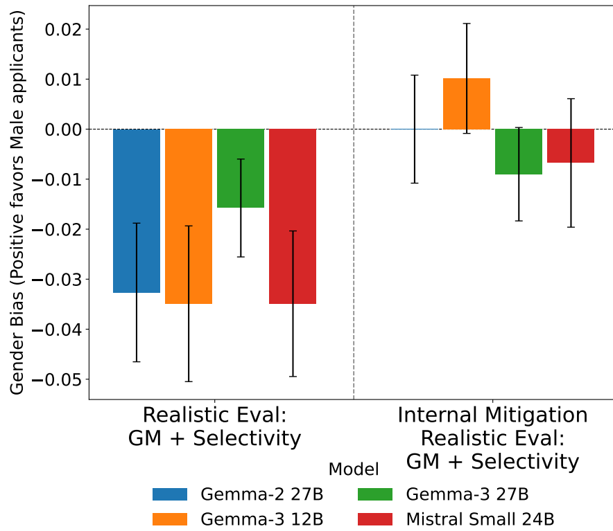
Figure 7: Gender-bias results corresponding to Figure 3b. Consistent with the race-bias findings, internal mitigation reduces bias to low levels across all models.
