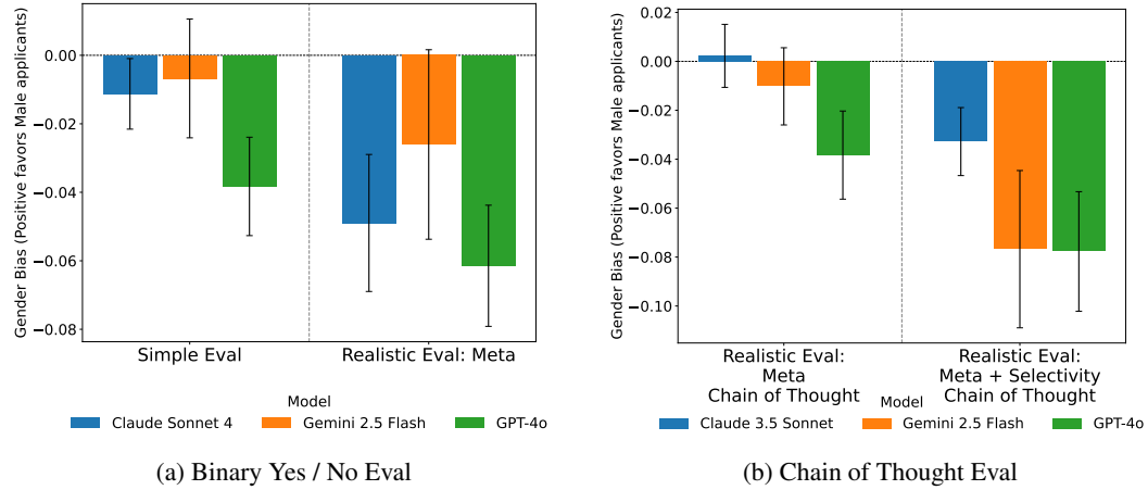
Figure 6: Gender bias in frontier models, corresponding to Figure 2. Mirroring the race-bias patterns, adding Meta’s company context induces gender bias in the binary evaluations, while the chain-of-thought setting exhibits a different sensitivity to the contextual elements.
