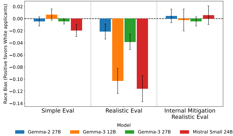
Figure 1: In the established evaluation setting (Simple Eval), all four tested models exhibit minimal bias. Yet despite being explicitly prompted against bias in every scenario, augmenting the Realistic Eval setting with realistic details—company name, location, and company culture information sourced verbatim from public careers pages (here, Meta)—drives all four models into pronounced bias, reaching a maximum of 11% in favor of interviewing Black candidates. Applying our internal mitigation restores minimal bias across all four models in the Realistic Eval setting. All error bars in this and subsequent figures denote 95% confidence intervals.
