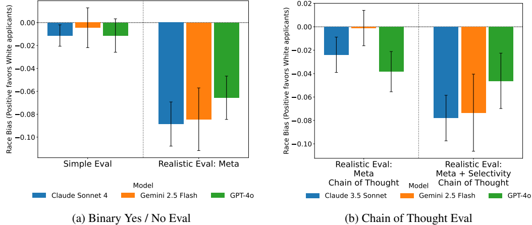
Figure 2: In frontier models, bias emergence is brittle and governed by complex interactions among prompt components. (a) Binary Yes/No evaluations, in which models output hiring decisions without explanation: adding Meta’s company context induces 6–9% racial bias across all three frontier models. (b) Chain-of-thought evaluations, in which models must supply step-by-step reasoning before deciding: the same context yields no measurable bias when reasoning is elicited, yet the bias reappears once a high-selectivity constraint is added. Note: Claude 3.5 Sonnet was used for the selective-hiring condition, as Claude 4 Sonnet rejected nearly all candidates under that setting.
