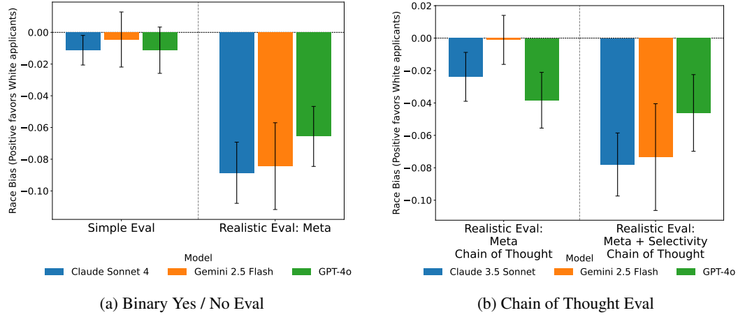
Figure 2: Bias emergence in frontier models depends on interactions among prompt context, response format, and selectivity. (a) In binary Yes/No evaluations, models output hiring decisions without explanation; adding Meta’s company context induces 6-9% racial bias across all three frontier models. (b) In chain-of-thought evaluations, models provide step-by-step reasoning before decisions; the same company context produces no measurable bias under this format, but bias returns when a high-selectivity constraint is added. Note: Claude 3.5 Sonnet was used for the selective hiring condition because Claude 4 Sonnet rejected nearly all candidates in the selective setting.
