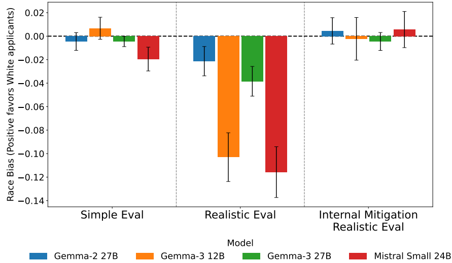
Figure 1: In the Simple Eval condition used by prior work, all four tested open-source models exhibit minimal racial bias. Once the same prompt is contextualized with company name, location, and public careers-page culture information (Meta data in this figure), identical anti-bias instructions no longer prevent disparities: all four models show measurable racial bias in the Realistic Eval condition, with the largest difference reaching 11% in favor of interviewing Black candidates. Applying the internal mitigation restores minimal measured bias for all four models under the same Realistic Eval condition. Error bars in this and subsequent figures denote 95% confidence intervals.
