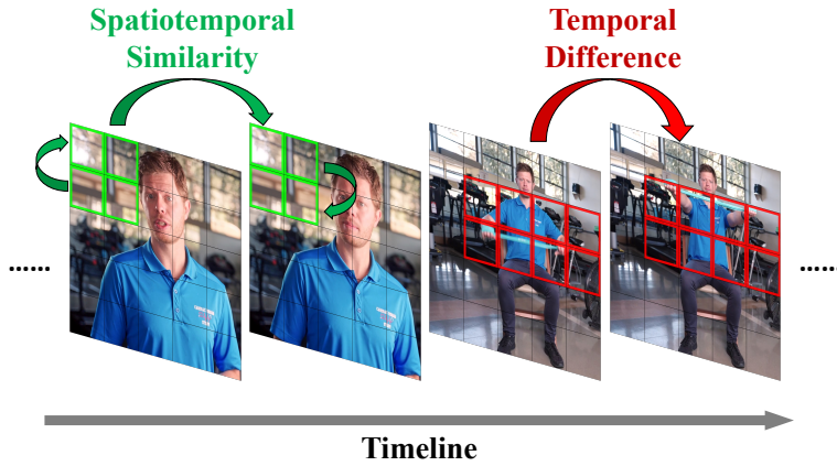
Figure 1: Core motivation of ST-SimDiff. Efficient video understanding requires the joint treatment of spatiotemporal similarity and temporal difference: similarity (left) supports compression of redundant information within frames and across adjacent frames, whereas difference (right) identifies key actions or events that define the video trajectory.
