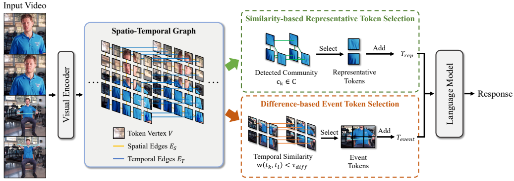
Figure 2: Overview of the ST-SimDiff framework. The pipeline proceeds through three stages: Spatio-Temporal Graph Construction, which encodes the coupled spatial and temporal token relationships within a single graph; Similarity-based Representative Token Selection, which compresses redundant, stable content via community detection; and Difference-based Event Token Selection, which localizes and preserves the tokens marking key dynamic transitions. The two selection paths operate in parallel and their outputs are merged, so that one compact subset simultaneously encodes what persists and what changes.
