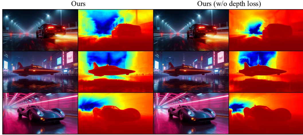
Figure 11: Depth loss ablation. 3DGS renderings and their corresponding depth maps. Adding the depth loss as auxiliary supervision prevents flattened geometry without sacrificing visual quality.
