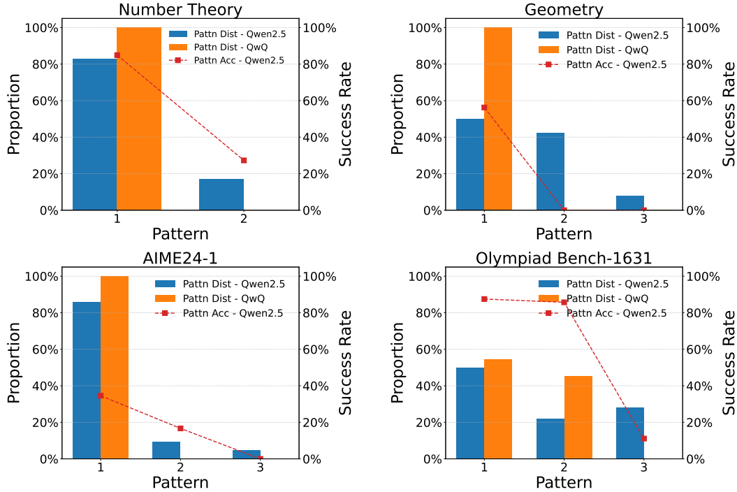
Figure 5: Evaluation on the larger models Qwen-2.5-32B and QwQ-32B. QwQ’s reasoning patterns converge onto the most accurate pattern of Qwen-2.5, demonstrating that our theory extends cleanly to large-scale models.
