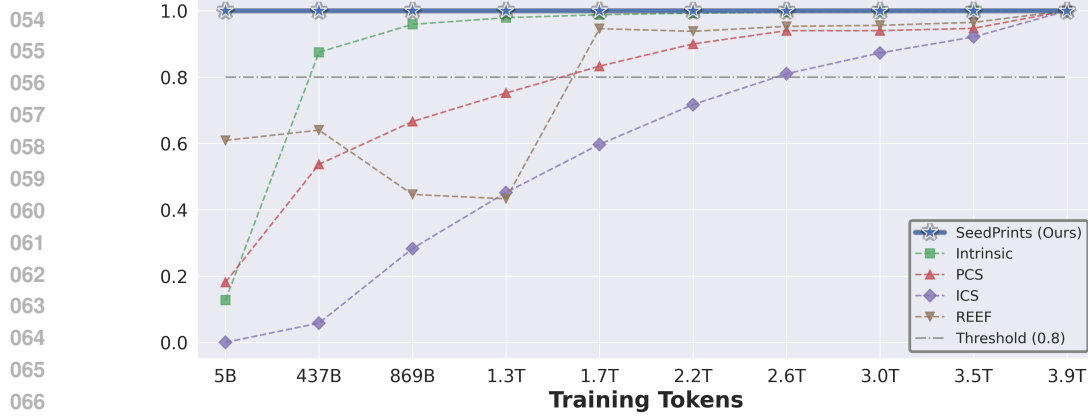
Figure 1: Existing fingerprinting methods fail to detect model lineage during early pretraining; SeedPrints detects it from the first checkpoint onward. We compare five methods on OLMo-2-7B checkpoints spanning 5B to 3.9T training tokens, each tested against the final checkpoint. The y -axis reports the similarity score (higher indicates a stronger lineage signal), and the dashed line marks the 0.8 detection threshold. Every baseline degrades and drops below the threshold at early checkpoints, exposing a systematic blind spot throughout the pretraining regime; SeedPrints , by contrast, attains perfect detection ( p \ll 0.001 , plotted as 1 - p ) from the very first checkpoint and remains saturated across the full trajectory.
