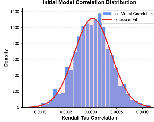
Figure 3: The empirical correlation distribution over \sim 2500 pairs of independently initialized models, evaluated on random inputs, closely matches a Gaussian centered at zero, directly validating the null model used in our test.
