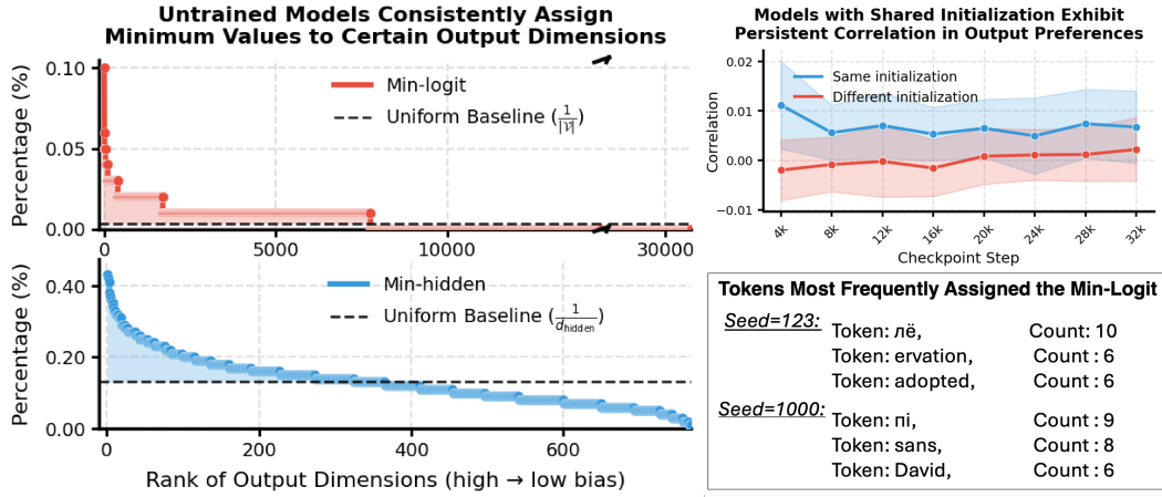
Figure 2: Initialization-born output bias persists through training. Left: Under completely random inputs, a randomly initialized LLaMA-2-style model produces highly non-uniform outputs: specific dimensions are systematically disfavored and therefore frequently receive the minimum value. This extreme bias appears in both logits (top, red) and final hidden representations (bottom, blue). The dashed line gives the expected frequency under a uniform distribution, and the arrows in the top panel mark a broken x-axis that omits low-frequency tail ranks. Upper Right: Training checkpoints retain weak input-wise correlation in output bias with the initialized model from which they descend. The correlation distribution is consistently shifted upward relative to correlations with independently initialized models, showing that initialization-born bias remains measurable after optimization. Lower Right: The most strongly biased dimensions are seed-dependent; the panel illustrates this effect using tokens that most frequently receive the minimum logit.
