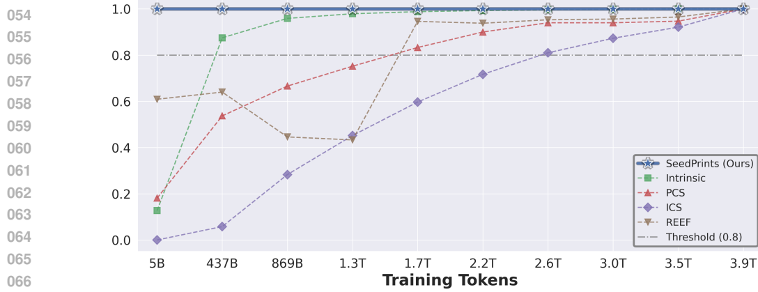
Figure 1: Existing fingerprinting methods fail to verify lineage during early pre-training. Five methods are evaluated on OLMo-2-7B checkpoints spanning 5B to 3.9T training tokens, with the final checkpoint serving as the reference model in every comparison. The y-axis reports the similarity score; larger values indicate stronger lineage evidence, and the dashed line denotes the 0.8 decision threshold used by similarity-based baselines. All baselines deteriorate on early checkpoints and fall below this threshold, whereas SeedPrints verifies lineage from the first checkpoint onward ( p \ll 0.001 , plotted as 1 - p ).
