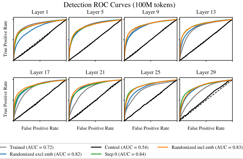
Figure 14: ROC curves for ‘detection’ auto-interpretability for Pythia-6.9b over 100 SAE latents. These results demonstrate the similarity in performance between the SAE variants.
