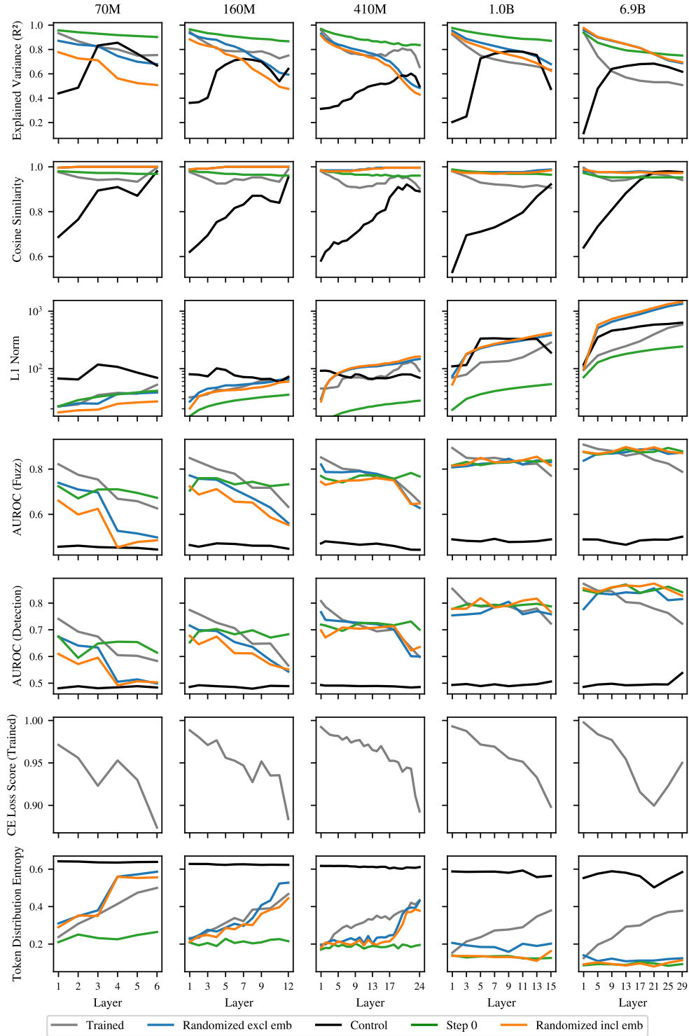
Figure 2: Comparison of sparse autoencoder evaluation metrics across Pythia models from 70M to 6.9B parameters. The trained and randomized variants exhibit similar trends across model scales, especially in larger models, whereas the control is consistently separated on several reconstruction-based metrics. These comparisons show that common aggregate SAE metrics often remain comparable despite substantial differences in transformer initialization.
